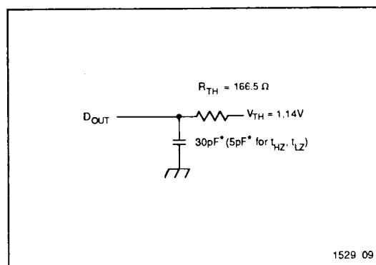
Figure 2. Thevenin Equivalent
