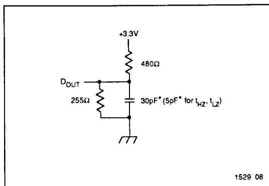
Figure 1. Output Load
