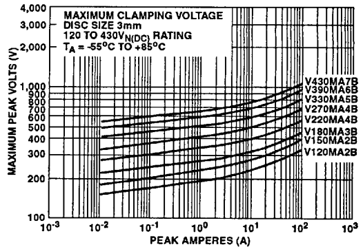
FIGURE 6. CLAMPING VOLTAGE FOR V120MA2B - V430MA7B
