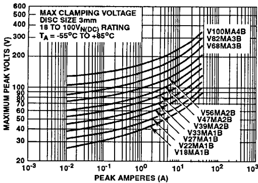
FIGURE 5. CLAMPING VOLTAGE FOR V18MA1B - V100MA4B
