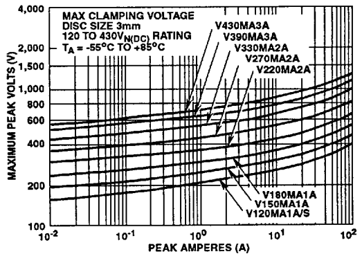
FIGURE 4. CLAMPING VOLTAGE FOR V120MA1A/S - V430MA3A
