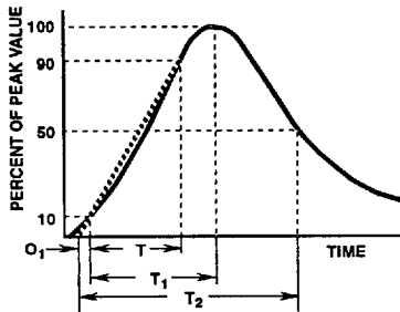
FIGURE 2. PEAK PULSE CURRENT TEST WAVEFORM
