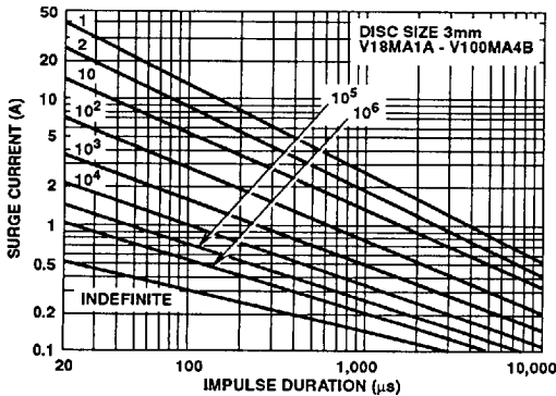
FIGURE 7. SURGE CURRENT RATING CURVES FOR V18MA SERIES - V100MA SERIES
