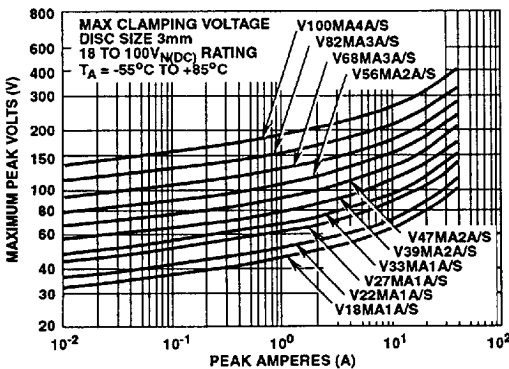
FIGURE 3. CLAMPING VOLTAGE FOR V18MA1A/S - V100MA4A/S
