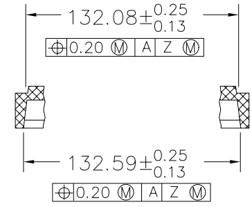
SECTION J-J
