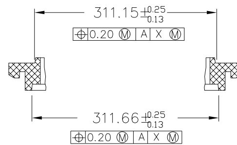
SECTION H-H
