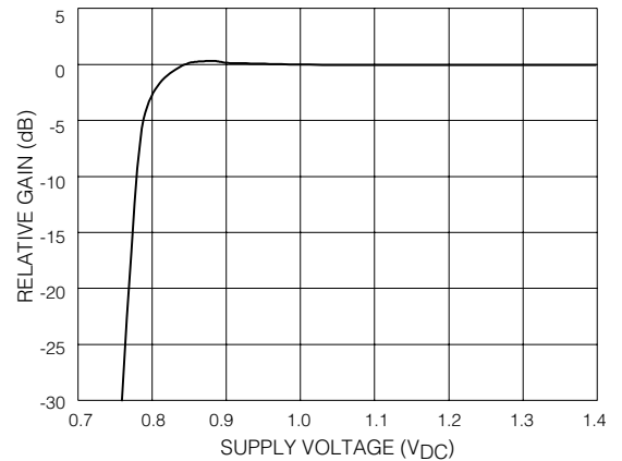
Fig. 7 Gain vs Supply Voltage
