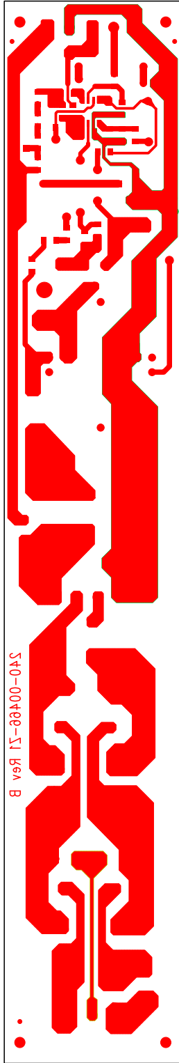
Figure 6. Circuit Routing (Bottom)
