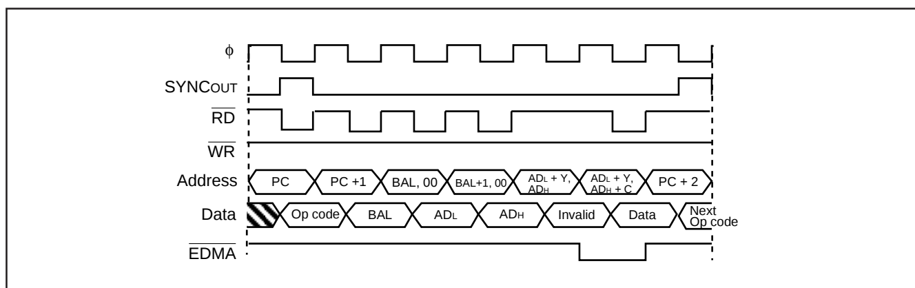
Fig. 69 LDA ($zz), Y instruction sequence when \overline{\text{EDMA}} enabled and T flag = "0"
