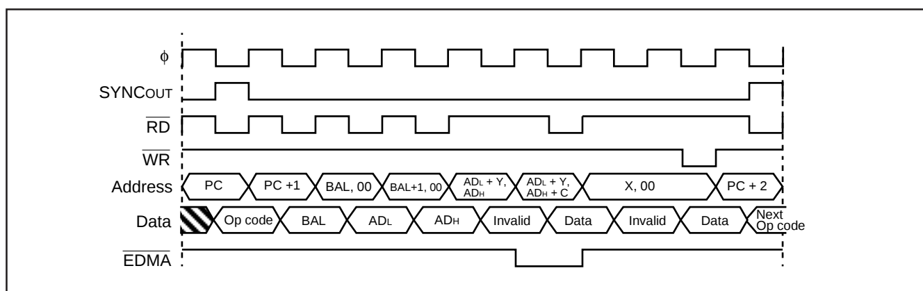
Fig. 70 LDA ($zz), Y instruction sequence when \overline{\text{EDMA}} enabled and T flag = "1"
