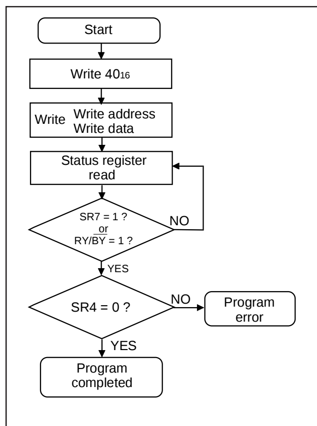
Fig. 81 Program flowchart
