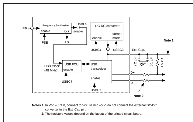
Fig.102 Peripheral circuit
