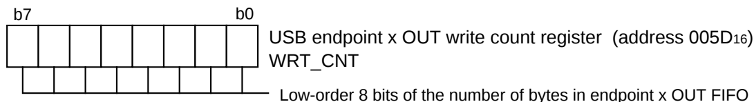
Fig. 48 Structure of USB endpoint x (x = 0 to 2) OUT write count registers
