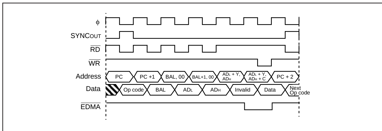
Fig. 68 STA ($zz), Y instruction sequence when \overline{\text{EDMA}} enabled
