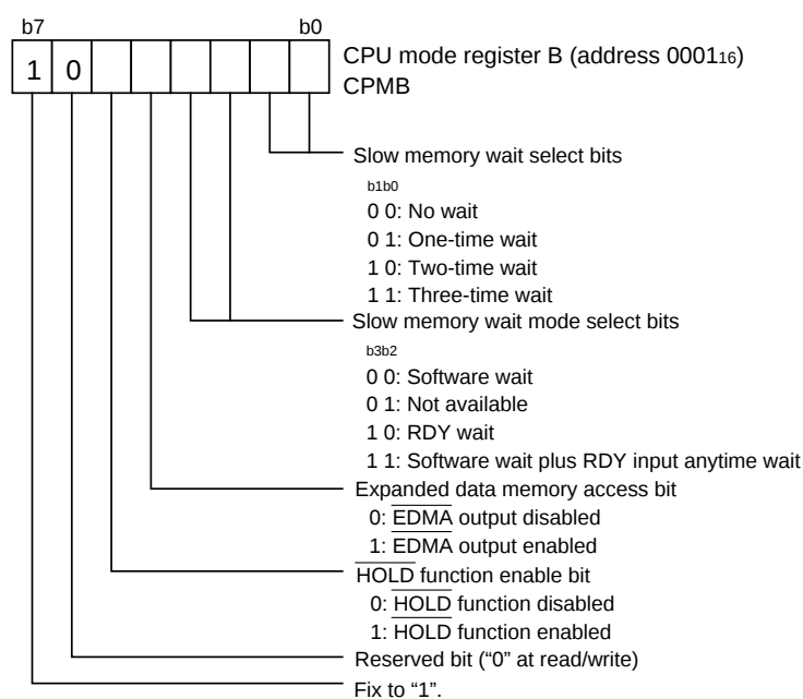
Fig. 8 Structure of CPU mode register
