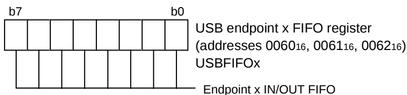
Fig. 49 Structure of USB endpoint x (x = 0 to 2) FIFO register
