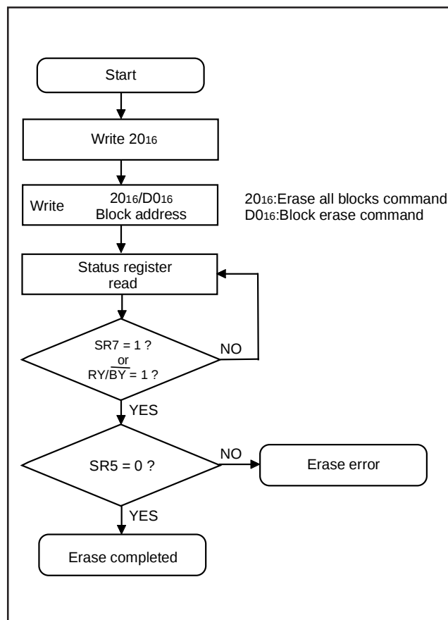
Fig. 82 Erase flowchart
