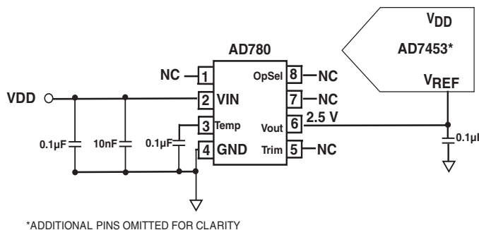
Figure 10. Typical V_{REF} Connection Diagram for V_{DD} = 5 V
