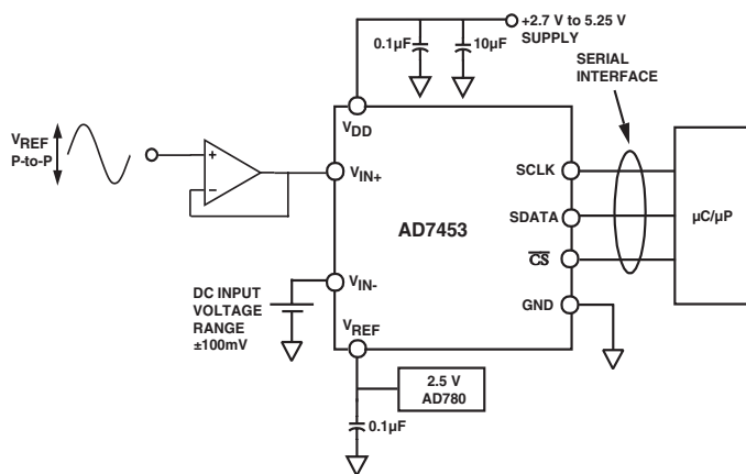
Figure 6. Typical Connection Diagram
