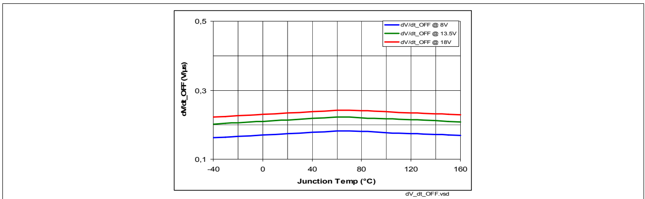
Figure 37 Slew Rate at Turn OFF - dV/dt_{OFF} = f(T_J; V_{GS}) , R_L = 4 \Omega
