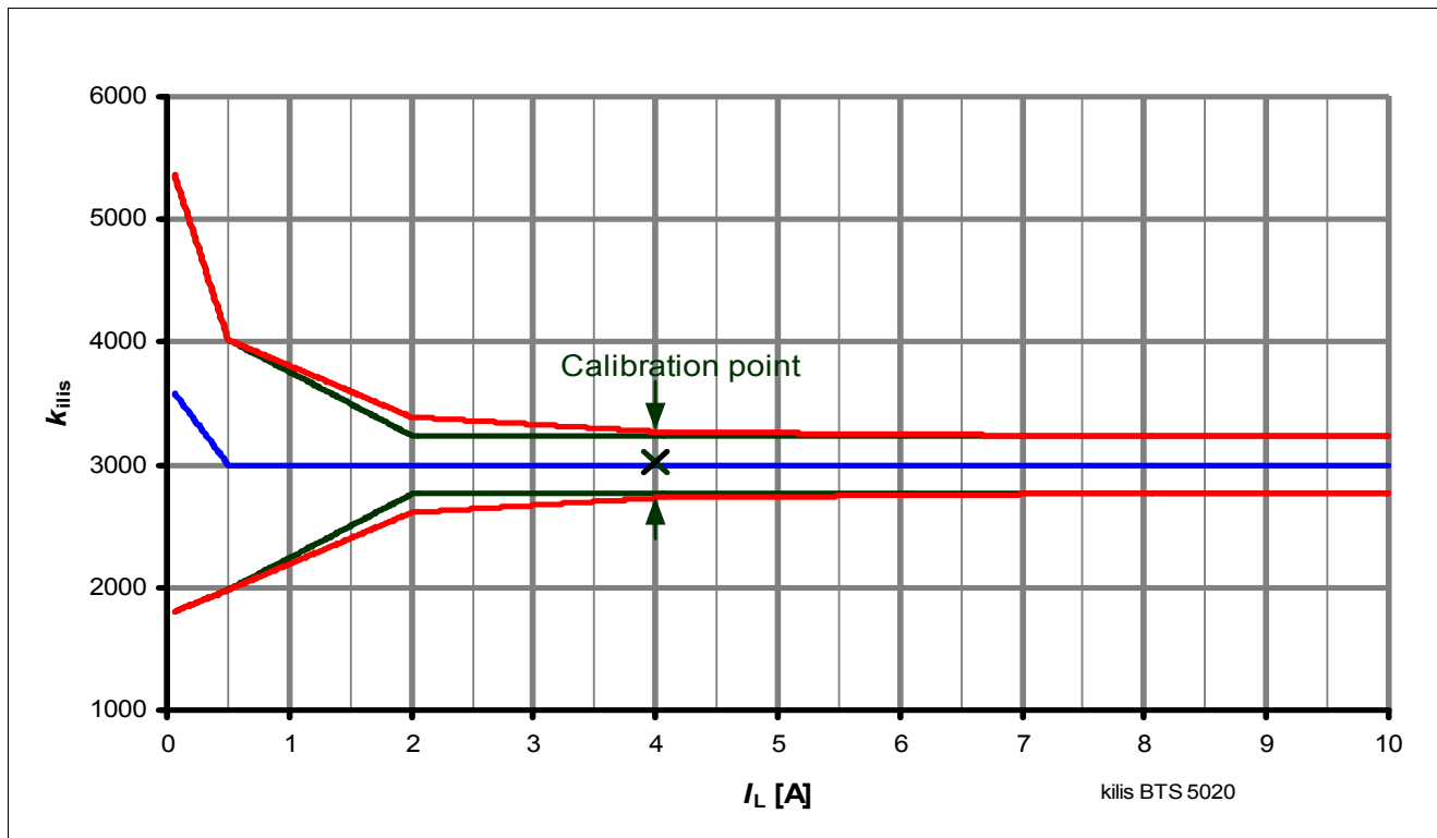
Figure 22 Improved SENSE Accuracy with One Calibration Point
