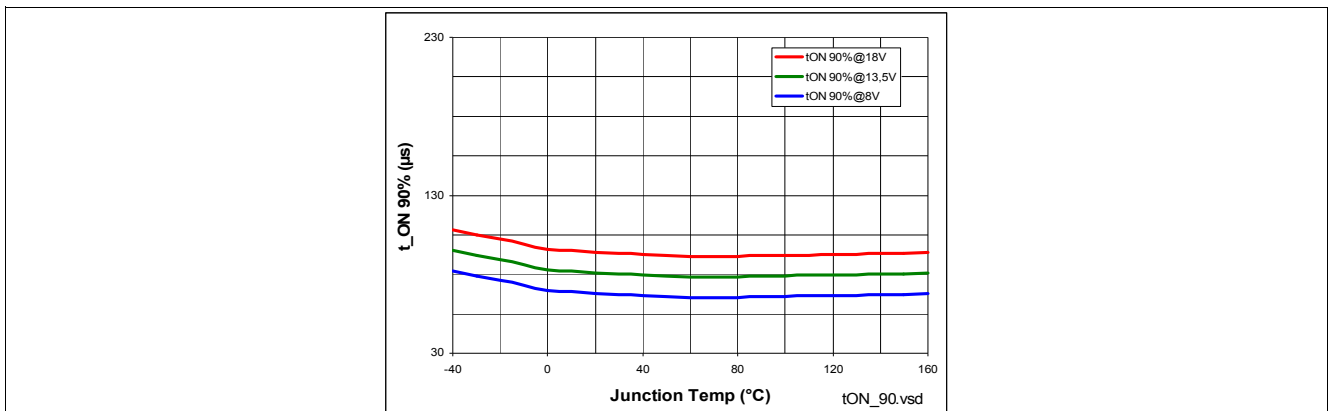
Figure 38 Turn ON t_{ON} = f(T_J; V_{GS}) , R_L = 4 \Omega
