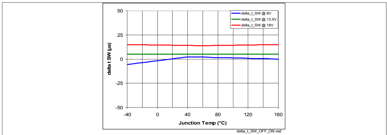
Figure 40 Turn ON / OFF matching \Delta t_{\text{SW}} = f(T_J; V_S) , R_L = 4 \Omega
