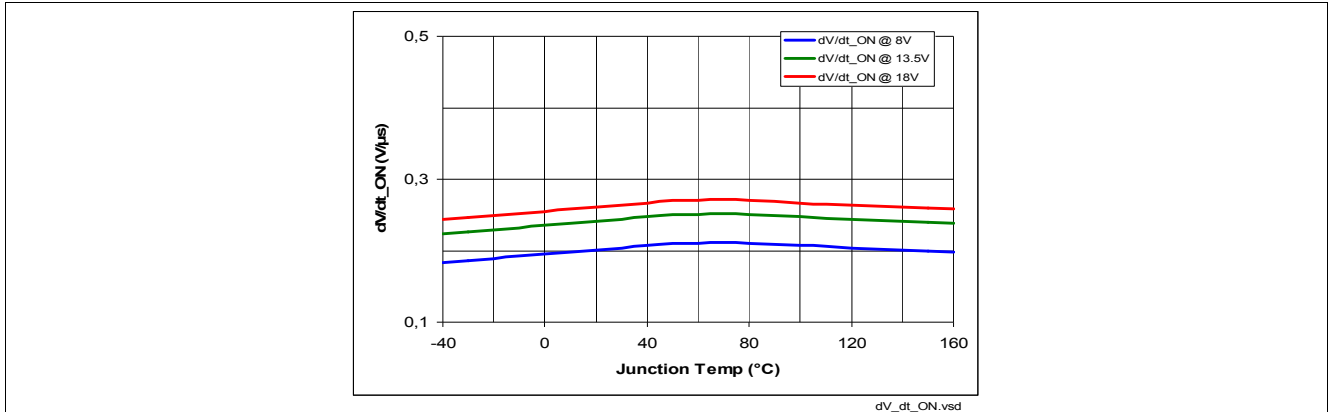
Figure 36 Slew Rate at Turn ON dV/dt_{ON} = f(T_J; V_{GS}) , R_L = 4 \Omega
