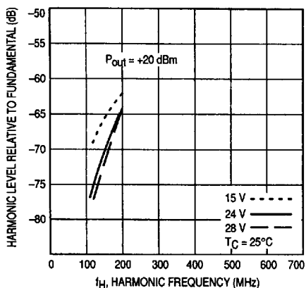
Figure 7. Second Harmonic Distortion versus Voltage
