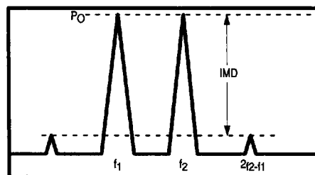
Figure 10. Intermodulation Test
