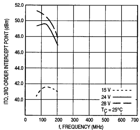
Figure 5. Third Order Intercept versus Voltage
