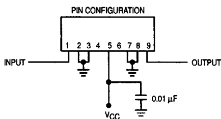
Figure 9. External Connections
