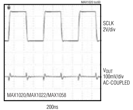
DAC DIGITAL FEEDTHROUGH ( R_{LOAD} = 10k\Omega , C_{LOAD} = 100pF , \overline{CS} = HIGH , DIN = LOW )
