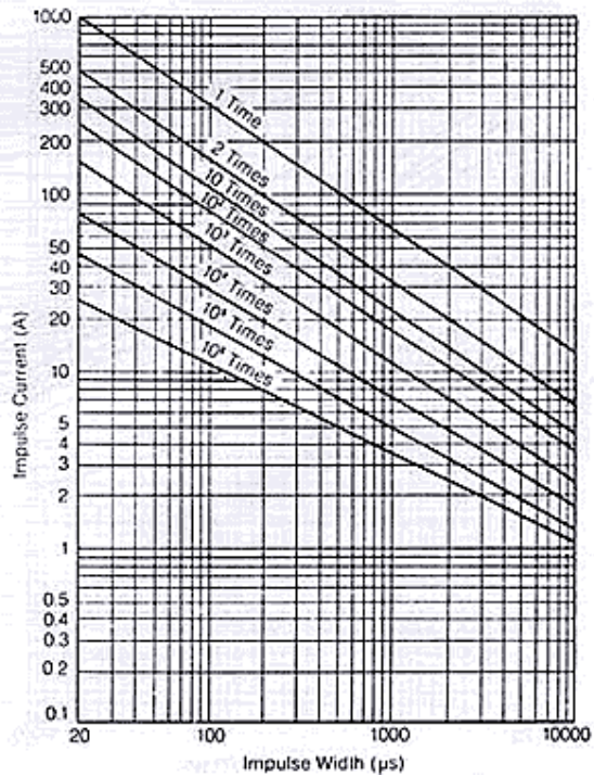
14 Series (CNR14D180K to CNR14D680K)
