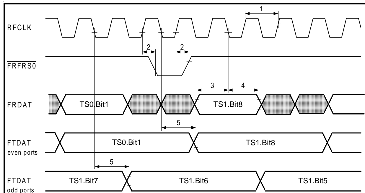
Figure 63 Framer Interface Timing in EC Mode
