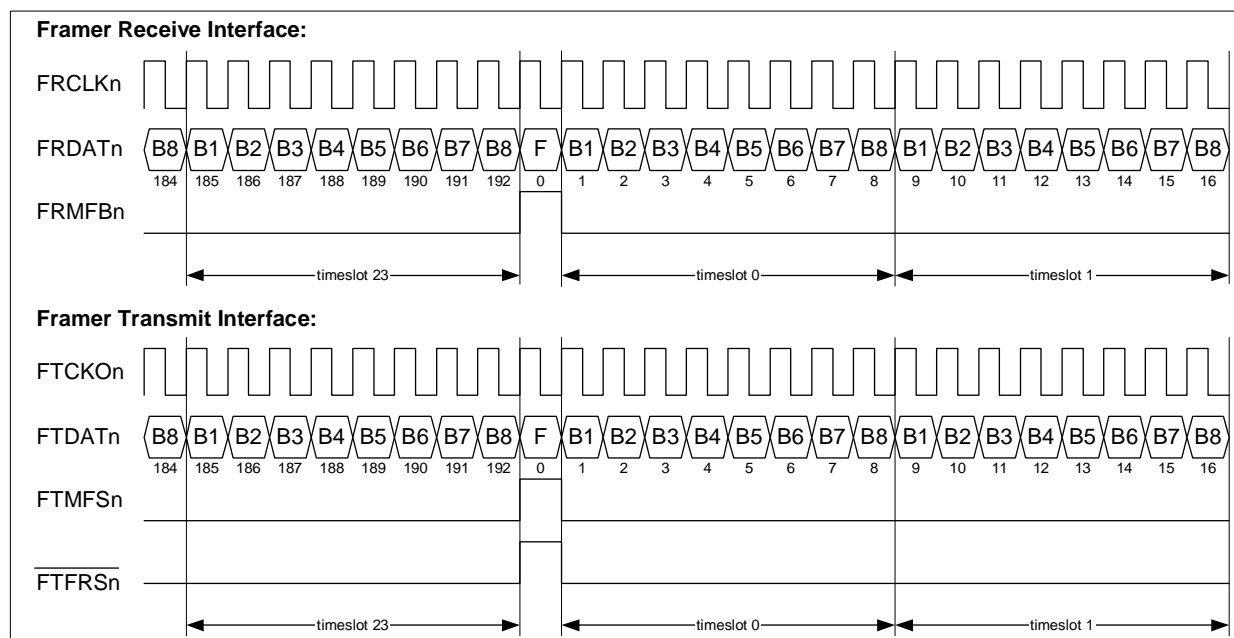
Figure 24 Framer Interface in GIM T1
