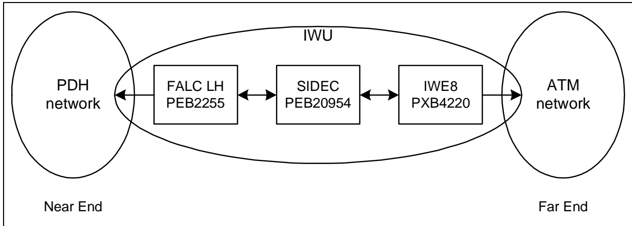
Figure 4 Echo Cancellation Application
