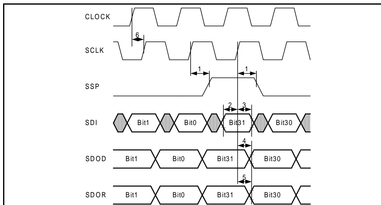
Figure 67 Clock Recovery Interface Timing Diagram
