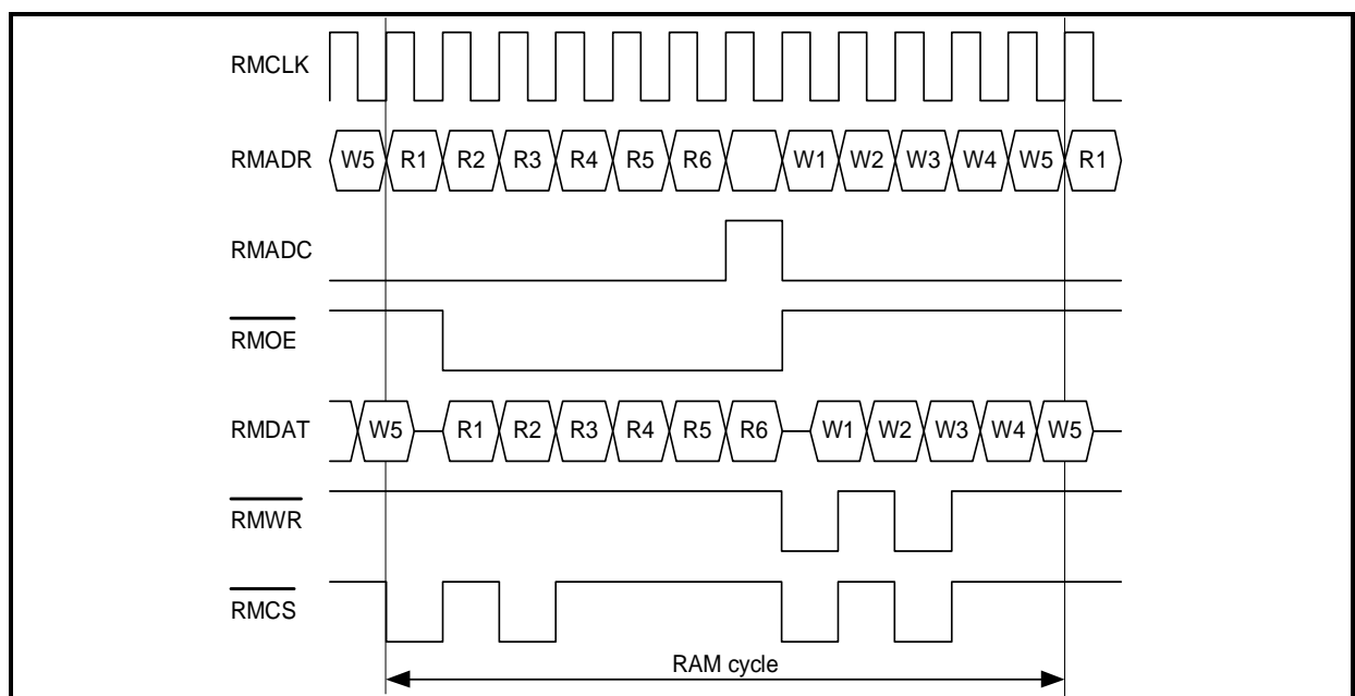
Figure 35 RAM Interface Protocol
