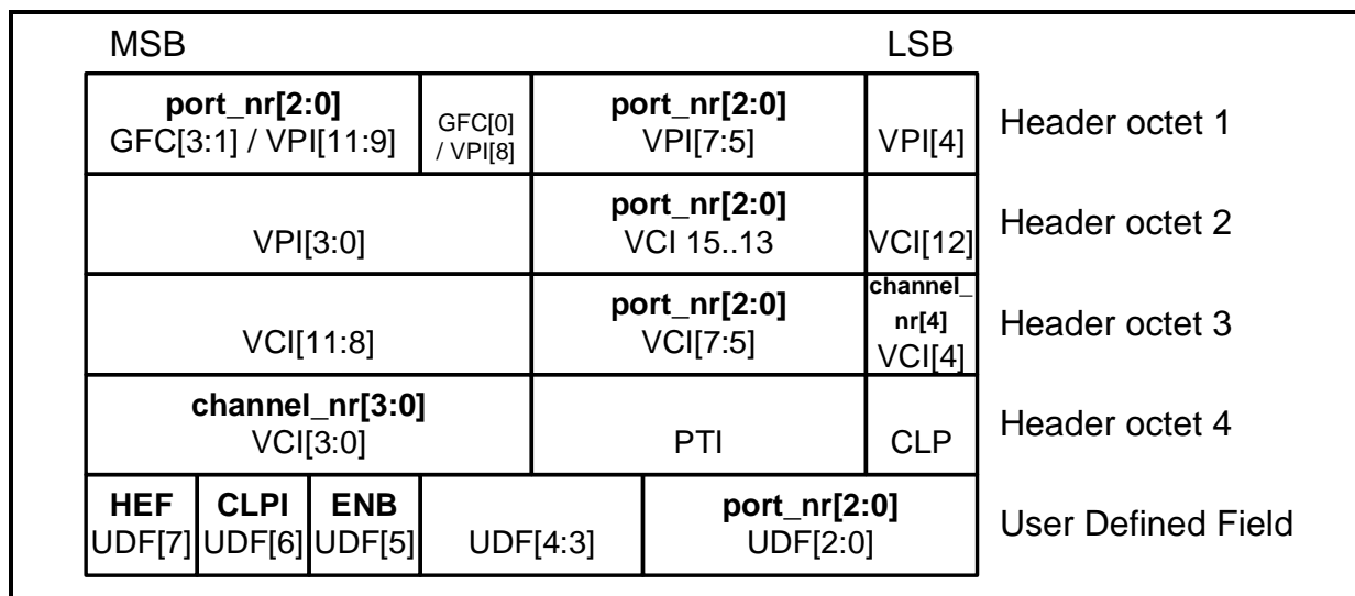
Figure 30 Utopia Sideband Signals
