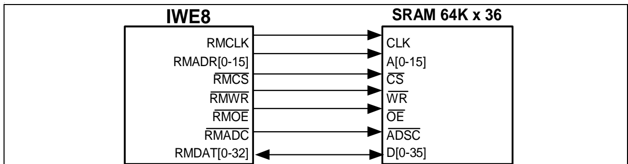
Figure 34 External RAM Connection
