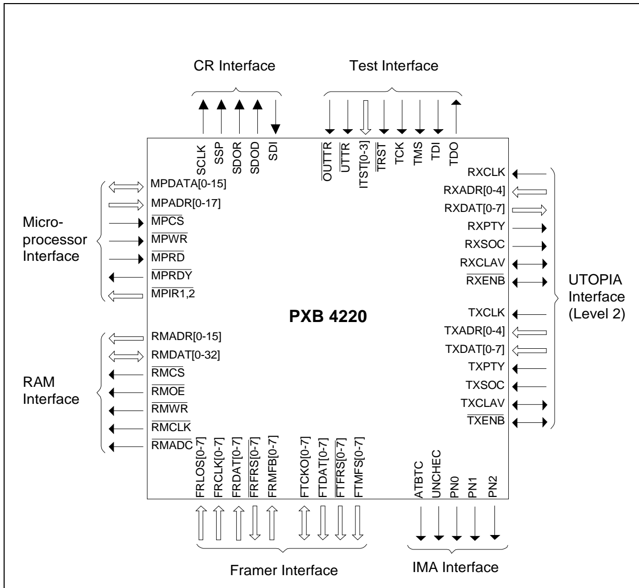
Figure 1 Logic Symbol
