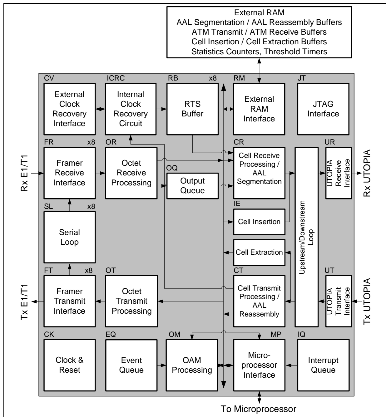
Figure 6 Block Diagram
