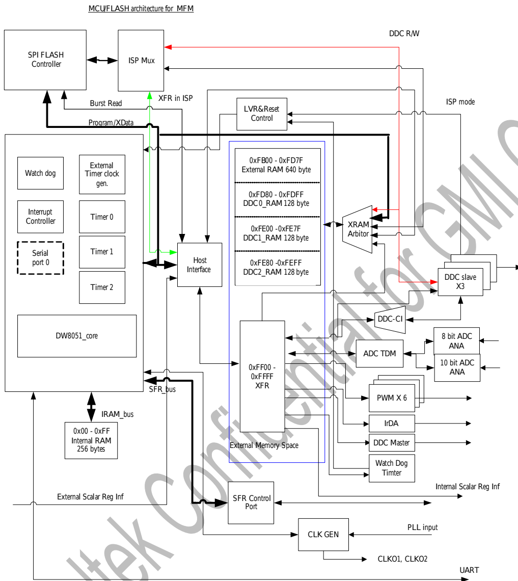
DW8051 micro-processor
