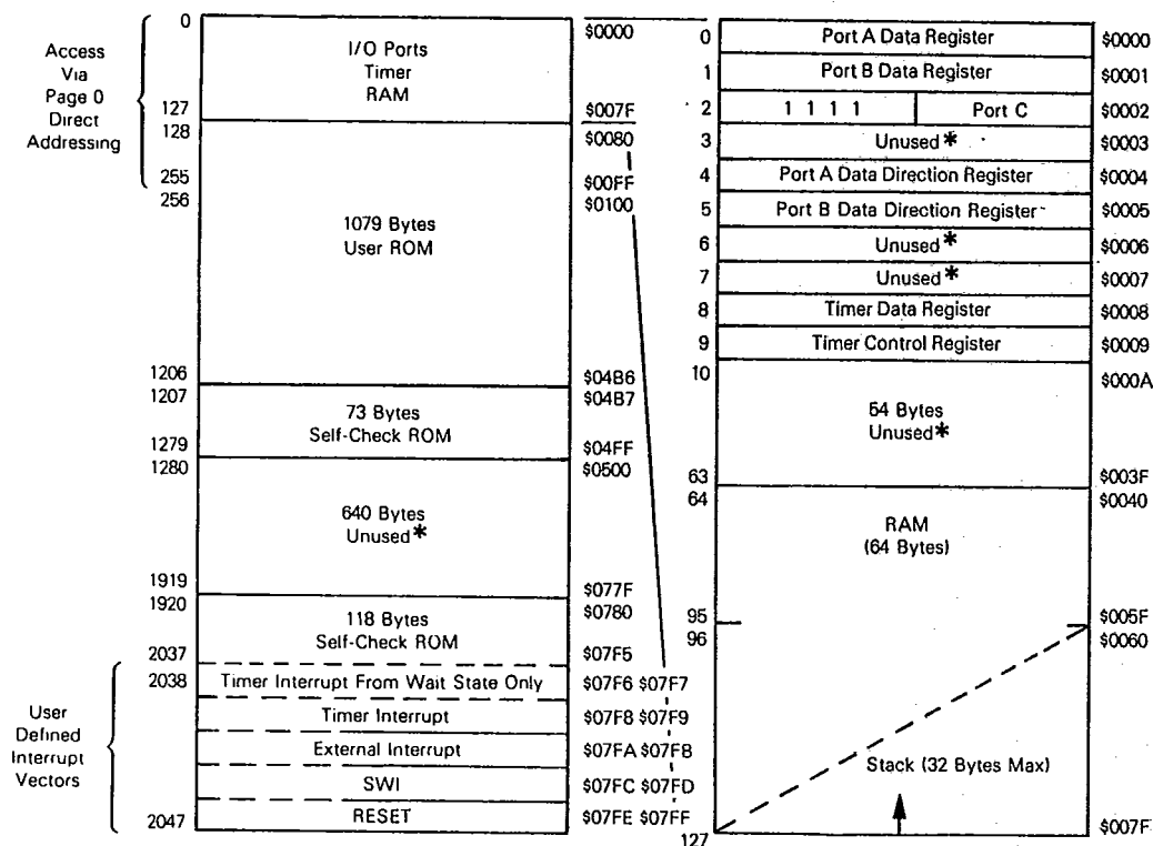
Fig. 11 - Address map.
