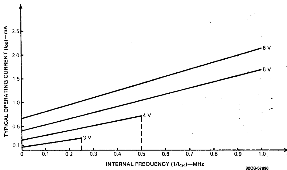
Fig. 3 - Typical operating current vs. internal frequency.
