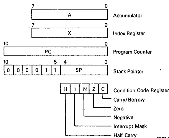
Fig. 12 - Programming model.
