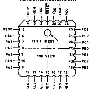
28-Lead Plastic Chip-Carrier Package (N Suffix)
