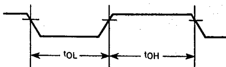
Oscillator Waveform
