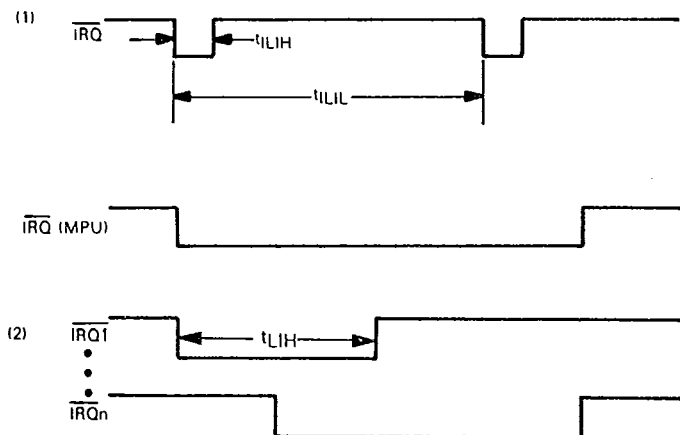
Fig. 15 - External Interrupt.
