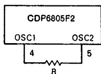
(b) RC Oscillator Connection
