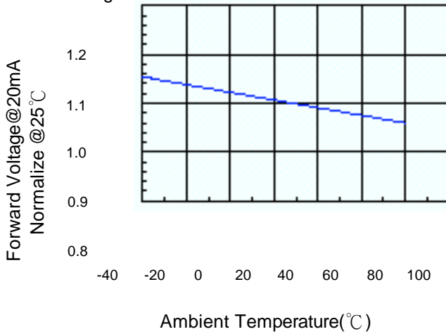
Fig.3 Forward Voltage vs. Temperature
