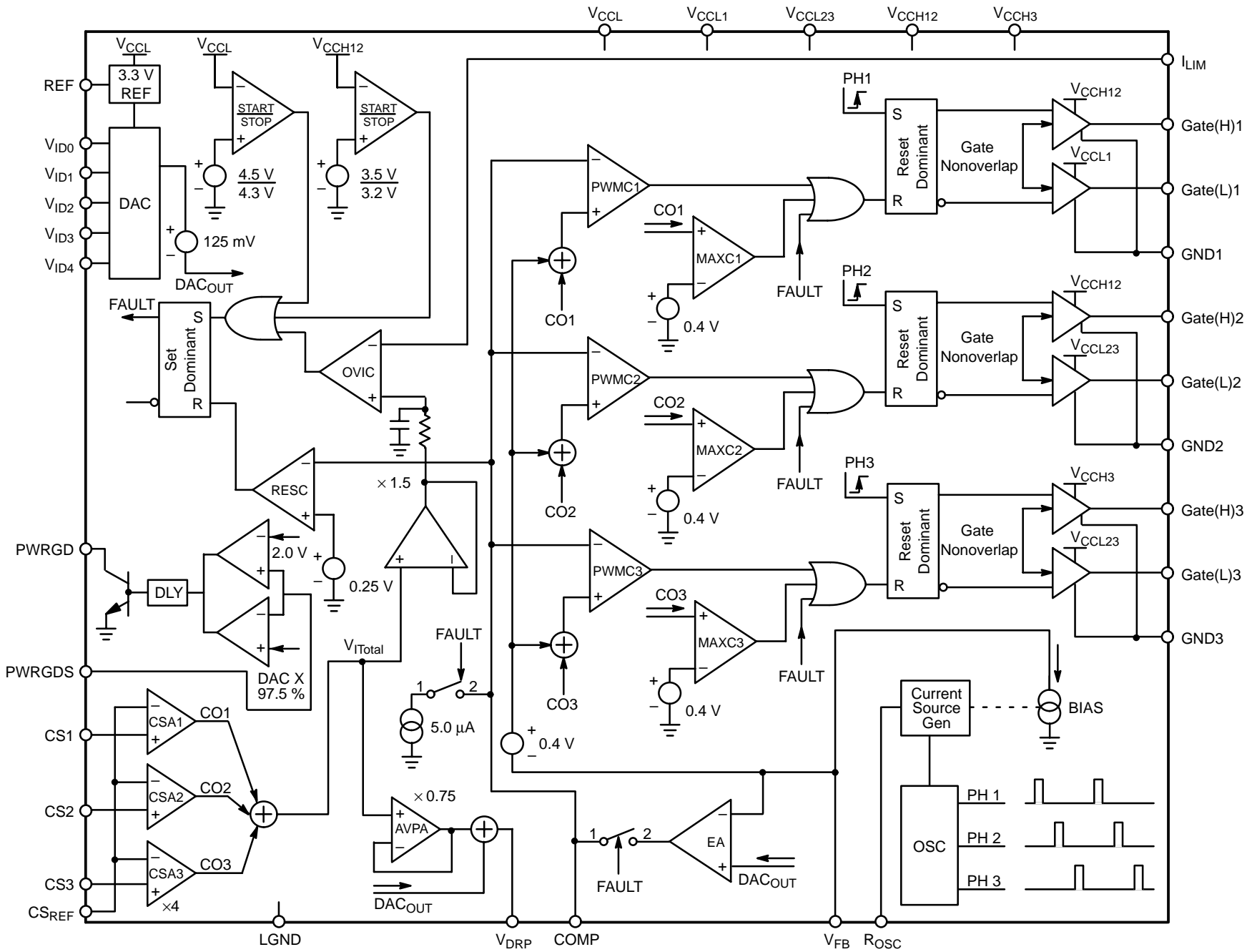
Figure 2. Block Diagram
