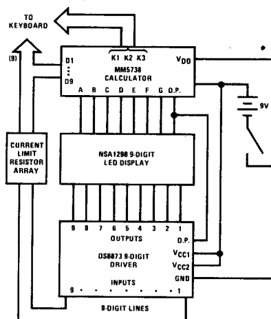
FIGURE 2. 9V System
