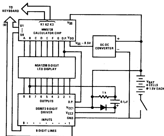
FIGURE 1. 4-Cell System
