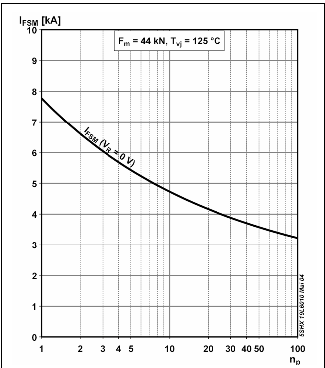
Fig. 12 Surge on-state current vs. number of pulses, half-sine wave, 10 ms, 50Hz
