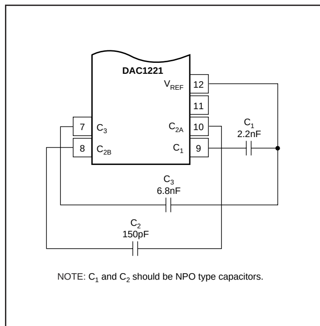
FIGURE 1. Capacitor Connections.
