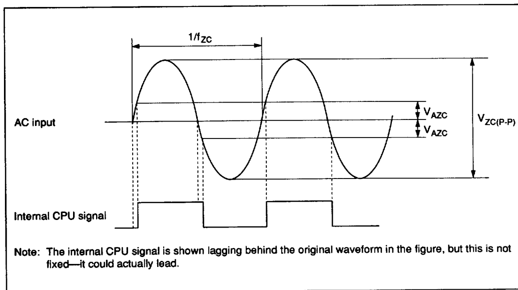
Figure 48 Zero-Crossing Detection
