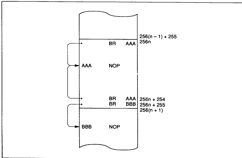
Figure 47 Branching when Branch Destination is on a Page Boundary
