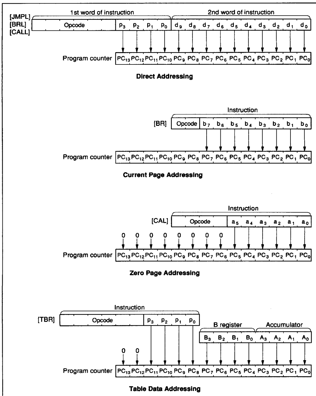
Figure 45 ROM Addressing Modes
