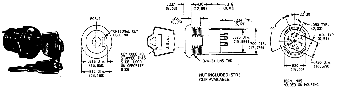
LOCK TYPE 'A' - 4 TUMBLER MOMENTARY
