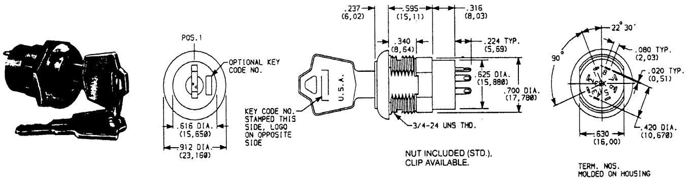
LOCK TYPE 'B' - 5 TUMBLER LOCK TYPE 'C' - 4 TUMBLER WITH DETENT
