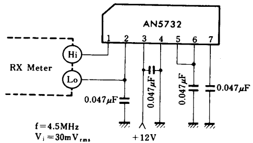
Test Circuit 2 (R i , C i )
