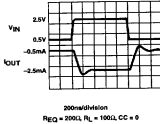
LSB Switching
