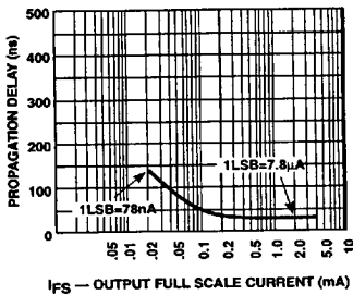
LSB Propagation Delay vs IFS
