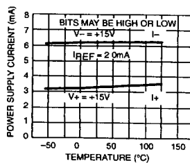
Power Supply Current vs Temperature
