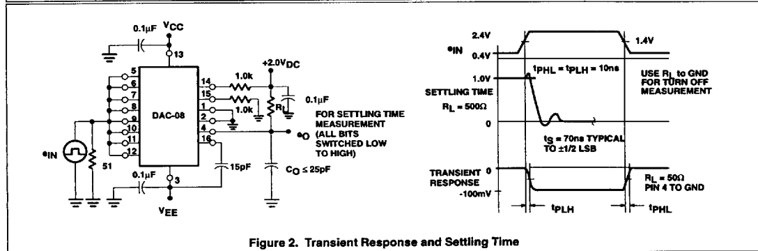
Figure 2. Transient Response and Settling Time
