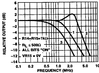
Reference Input Frequency Response
