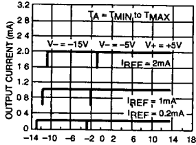
Reference AMP Common-Mode Range All Bits On
