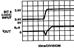
LSB Switching
