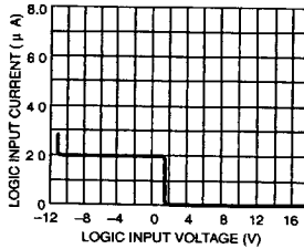
Logic Input Current vs Input Voltage
