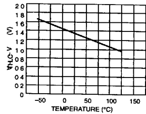
V TH - V LC vs Temperature
