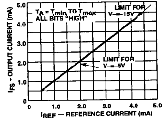
Full-Scale Current vs Reference Current
