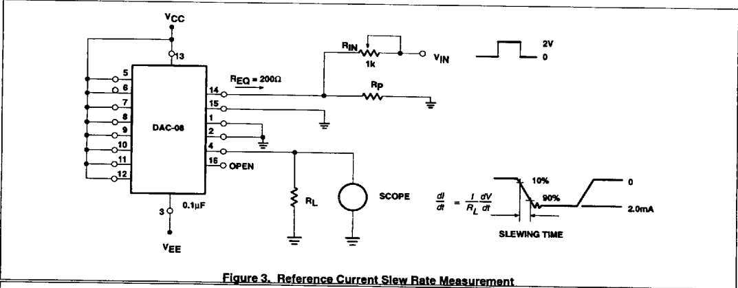
Figure 3. Reference Current Slew Rate Measurement
