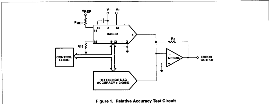
Figure 1. Relative Accuracy Test Circuit
