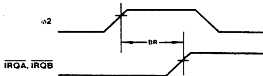
Figure 11. Interrupt Clear Timing
