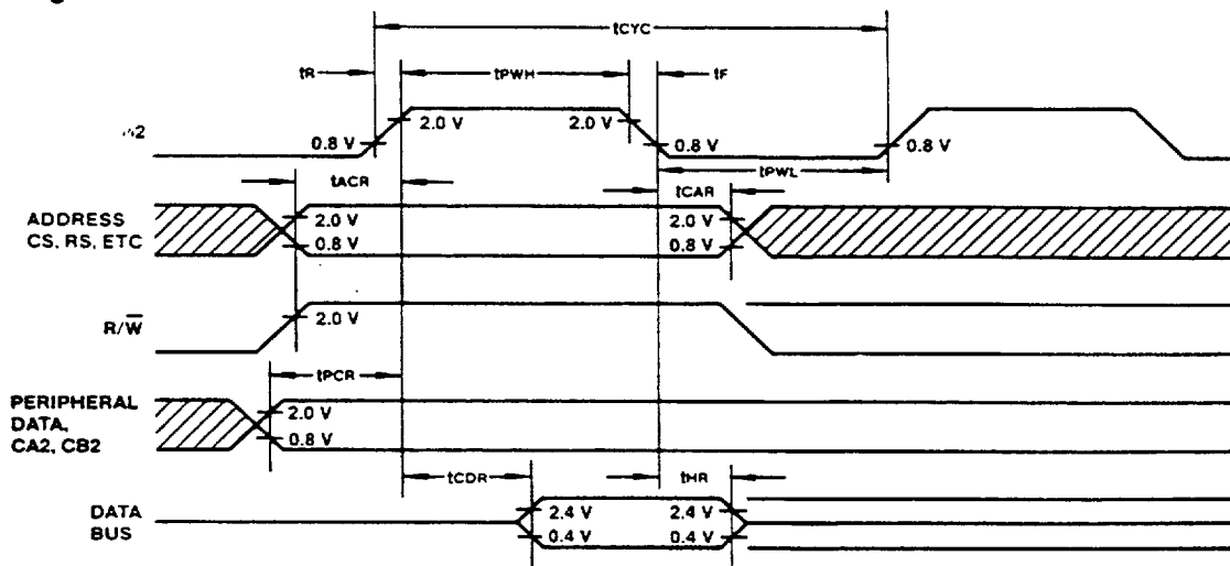
Figure 1. Read Timing
