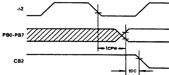
Figure 9. PB Port Delay Time
