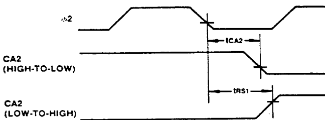
Figure 4. CA2 Timing
