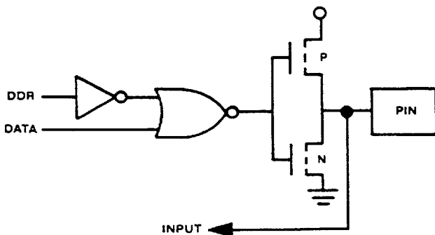
Figure 14. Port A Buffer Circuit (PA0-PA7)
