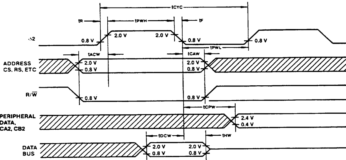
Figure 2. Write Timing
