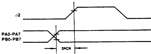
Figure 3. Peripheral Data Setup Time
