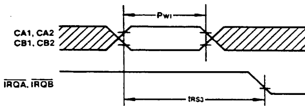
Figure 10. Interrupt Timing
