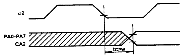
Figure 8. PA Port Delay Time
