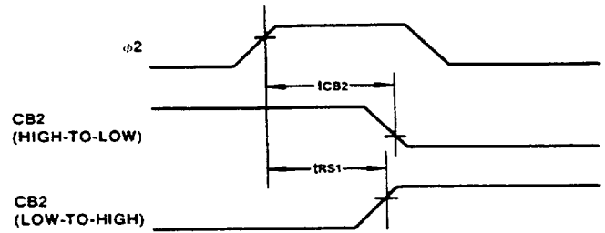
Figure 6. CB2 Timing
