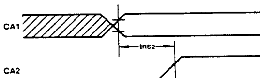
Figure 5. CA1/CA2 Timing
