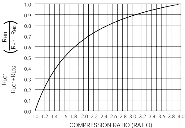
Fig. 8 Compression Settings Resistor Ratio for High Pass Channel ( R_{H11} & R_{H12} ) and Low Pass Channel ( R_{L01} & R_{L02} )
