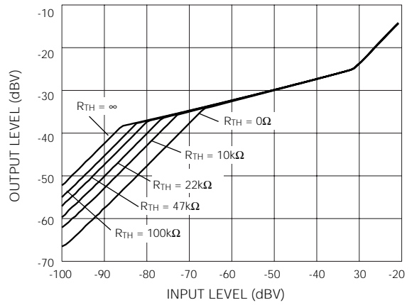
Fig. 11 I/O Transfer Function for Different RTH Resistors
