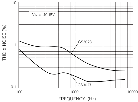
Fig. 18 THD and Noise vs Frequency
