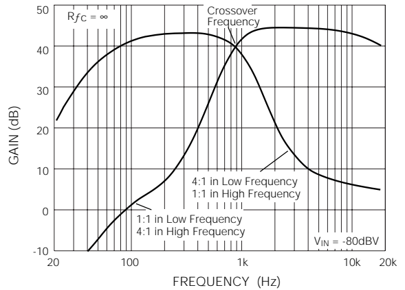
Fig. 15 Crossover Frequency Representation for GS3028 Processor
