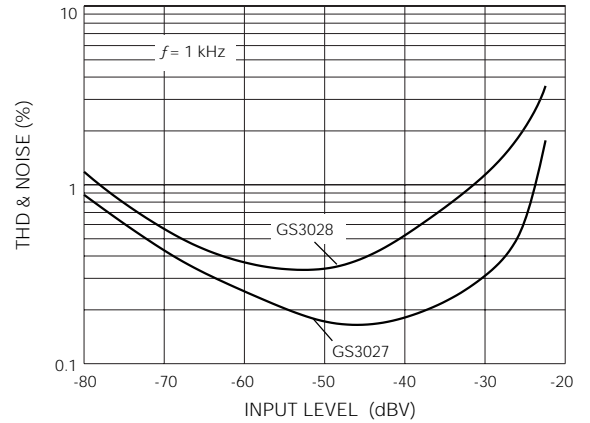
Fig. 19 THD and Noise vs Input Level
