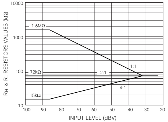
Fig. 13 Expander / Compressor Resistors Values
