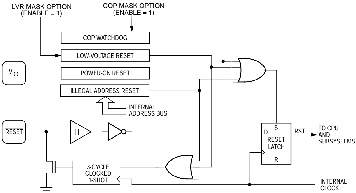
Figure 5-1. Reset Sources
