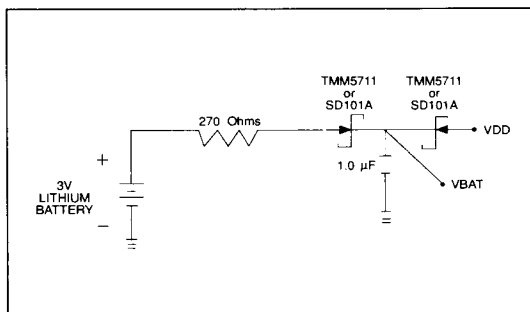
FIGURE 2-3A. VBAT EXTERNAL SUPPORT
