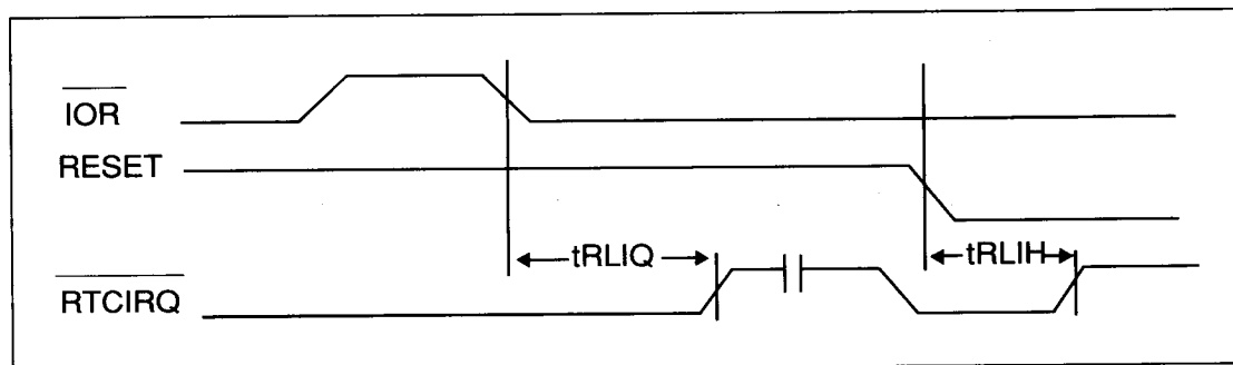
FIGURE 4-13. RTCIRQ RELEASE TIMING DIAGRAM
