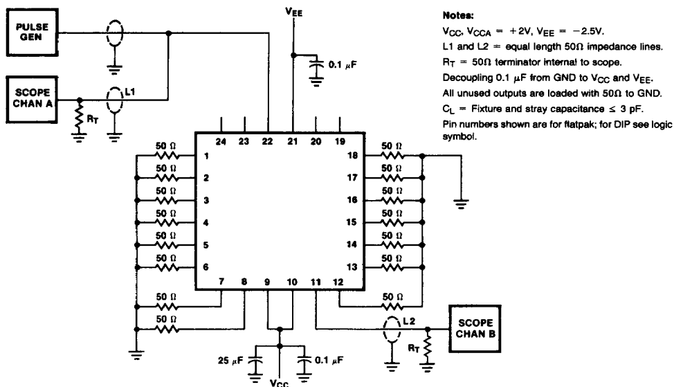
FIGURE 1. AC Test Circuit
