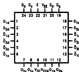
24-Pin Flatpak
