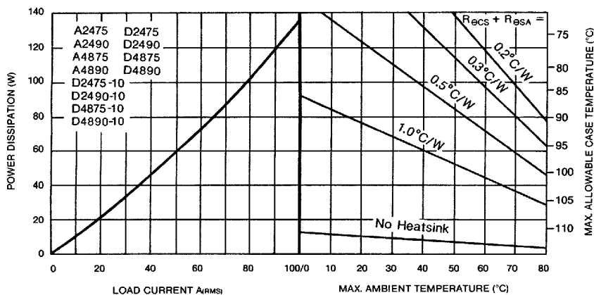
Figure 9. Thermal Derating Curves 75 &amp; 90 Amp., 240 and 480V.
