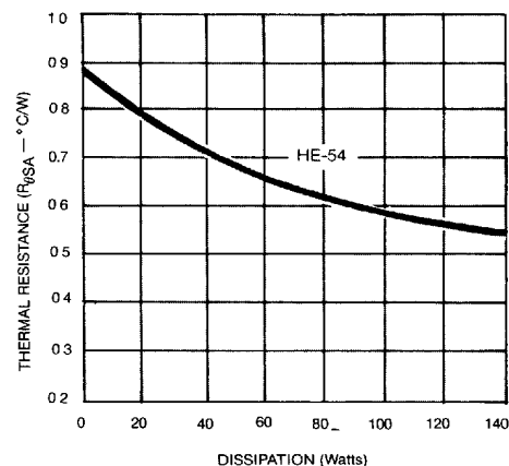
Typical Heat Sink Characteristics
