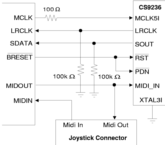
Figure 11. CS9236 Wavetable Serial Port Interface
