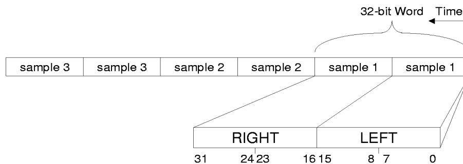
Figure 16. 16-bit Stereo, Signed Little Endian Audio Data
