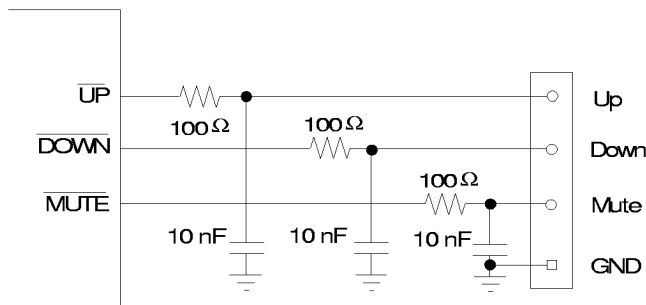
Figure 17. Volume Control Circuit
