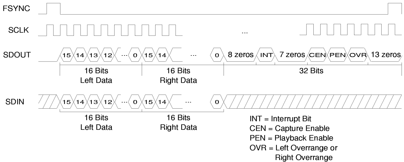
Figure 6. 64-bit Enhanced Mode (SF1,0 = 00)
