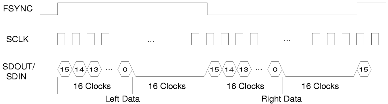
Figure 7. 64-bit Mode (SF1,0 = 01)
