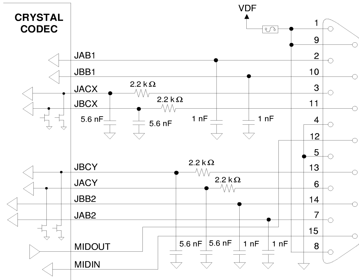
Figure 5. Joystick Logic
