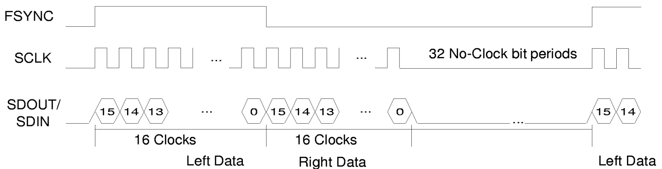
Figure 8. 32-bit Mode (SF1,0 = 10)
