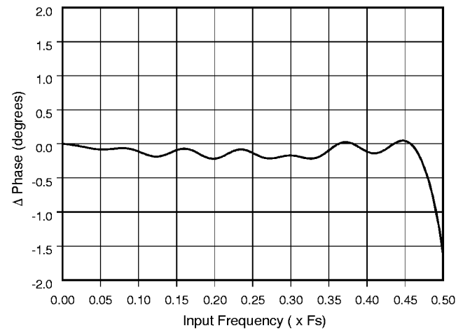
Figure 32. Deviation from Linear Phase
