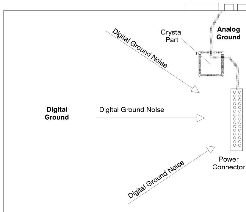
Figure 23. Suggested Motherboard Layout
