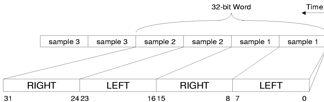
Figure 14. 8-bit Stereo, Unsigned Audio Data
