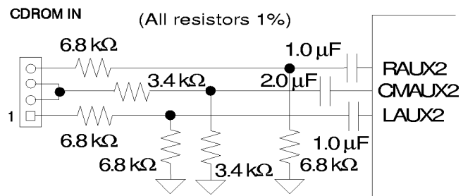
Figure 20. Differential CDROM In
