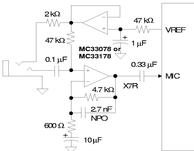
Figure 21. Microphone Input
