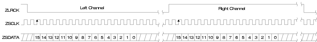
Figure 10. ZVPORT Clocking Format
