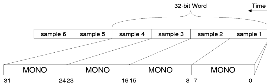
Figure 13. 8-bit Mono, Unsigned Audio Data
