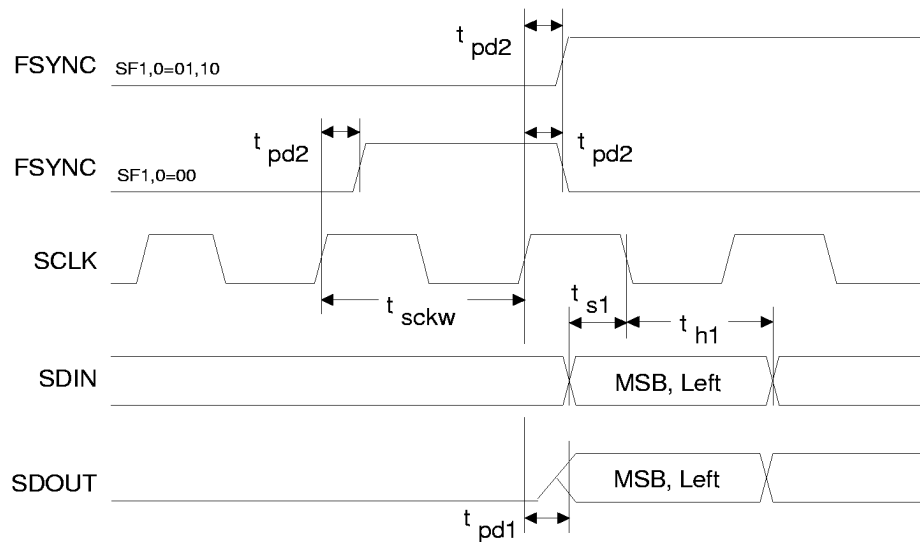
CS4610 DSP Serial Port Timing
