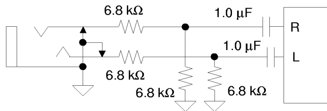
Figure 19. Line Inputs
