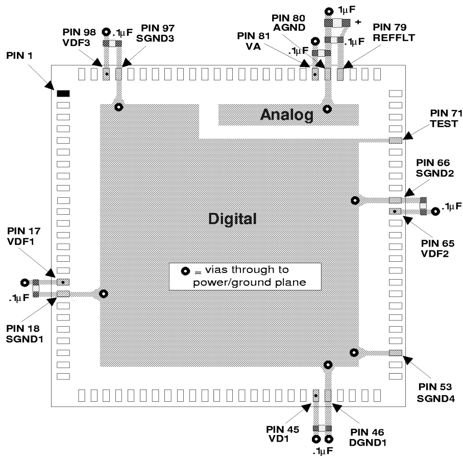
Figure 25. Recommended Decoupling Capacitor Positions
