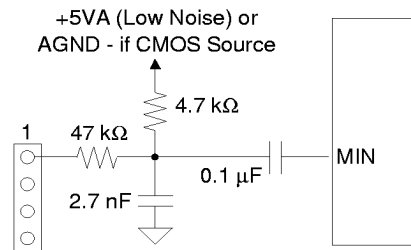
Figure 22. Mono Input
