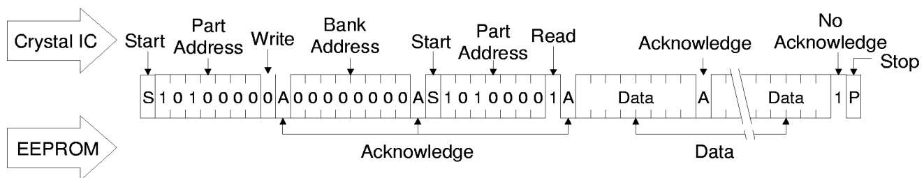
Figure 3. EEPROM Format
