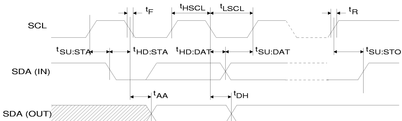
E²PROM 2-Wire Interface Timing
