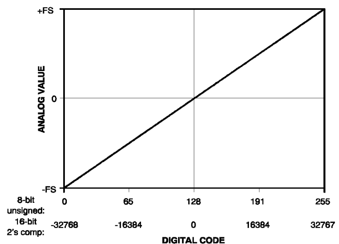
Figure 12. Linear Transfer Functions
