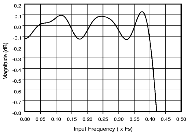
Figure 27. ADC Passband Ripple
