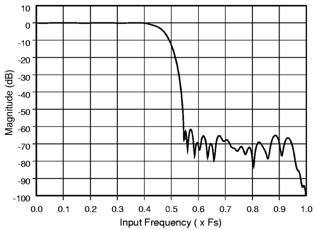
Figure 29. DAC Filter Response
