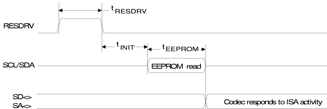
Reset Timing
