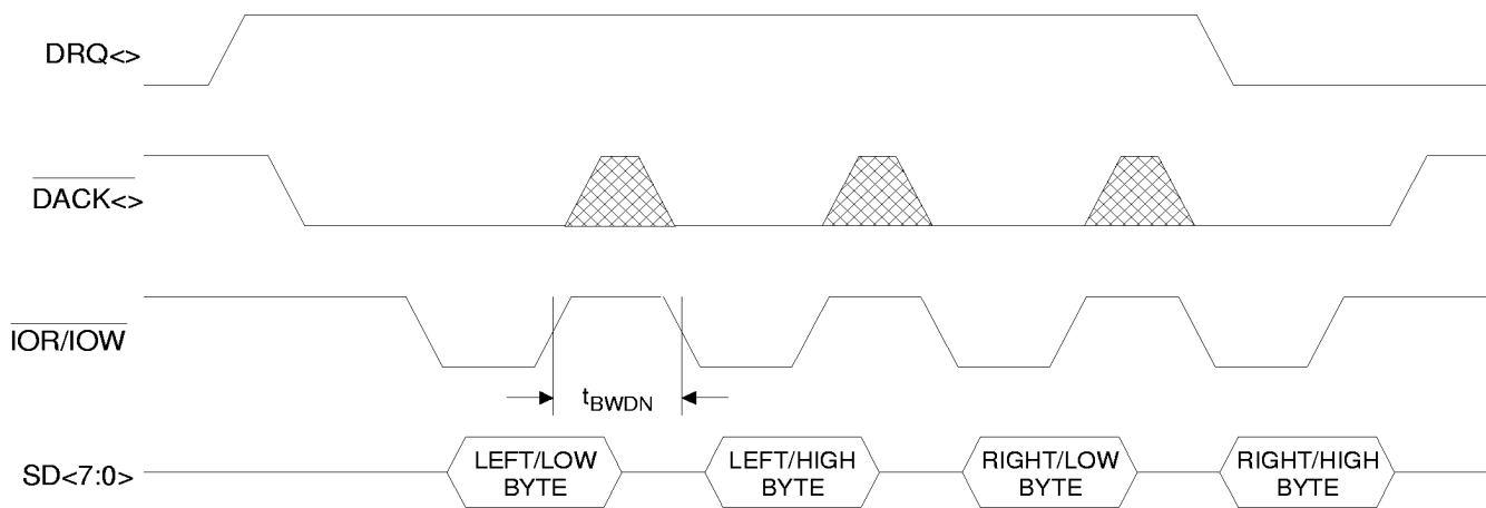
16-Bit Stereo DMA Cycle
