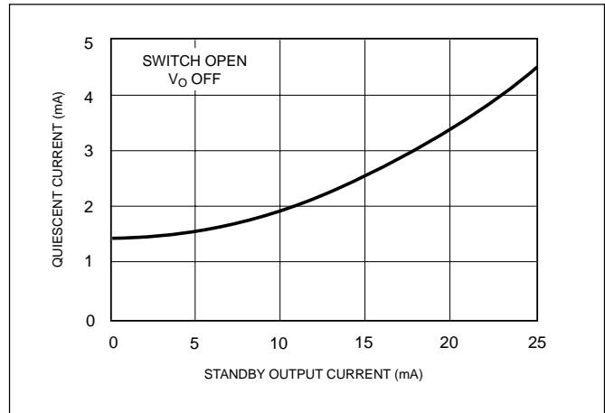
Quiescent Current vs. Standby Output Current
