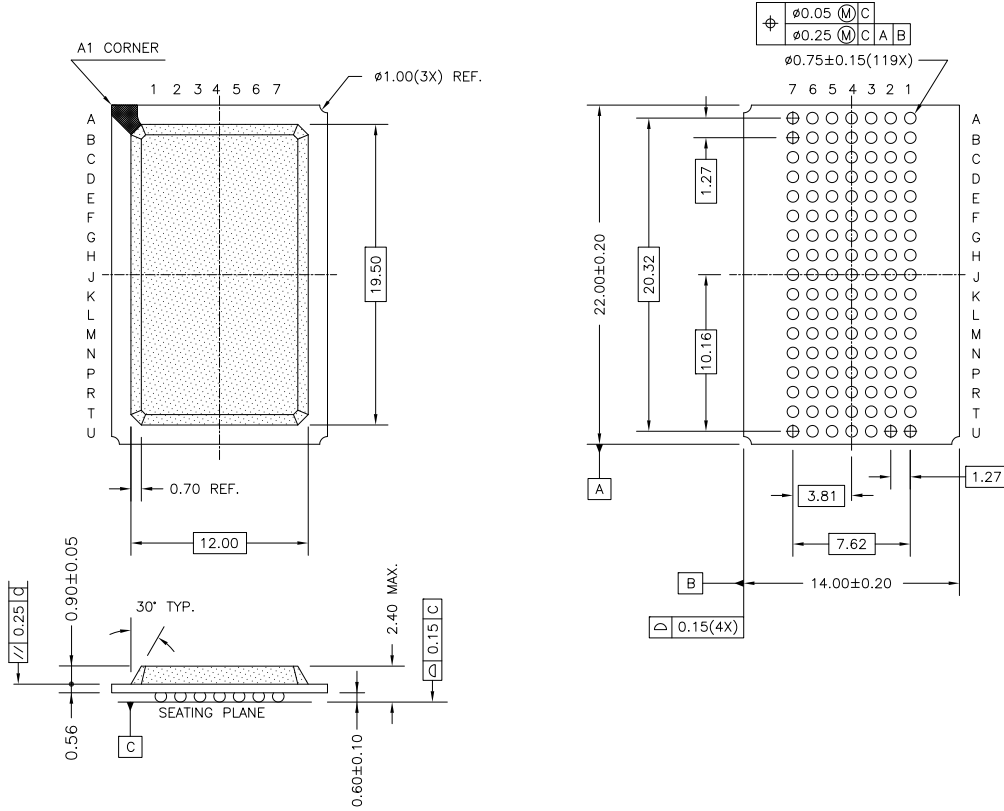
Figure 8. 119-ball PBGA (14 × 22 × 2.4 mm) BG119, 51-85115
