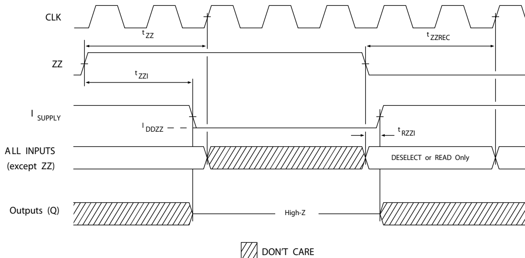
Figure 7. ZZ Mode Timing [32, 33]
