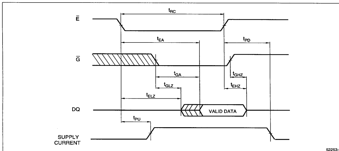
Figure 5. Read Cycle No. 2
