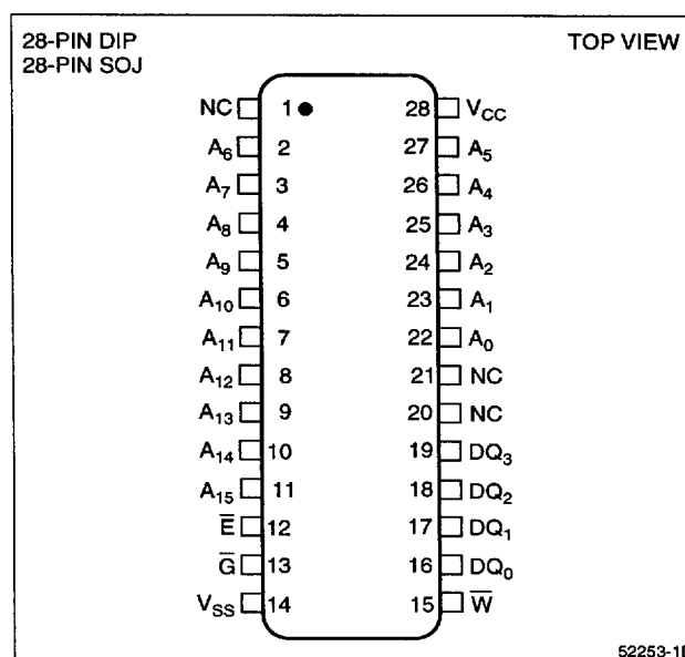
Figure 1. Pin Connections for DIP and SOJ Packages
