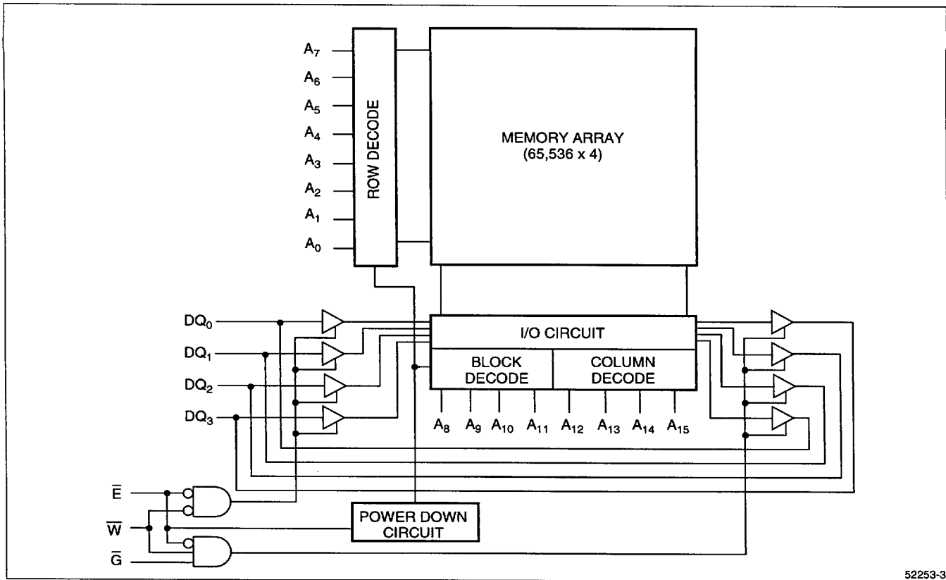
Figure 2. LH52253 Block Diagram
