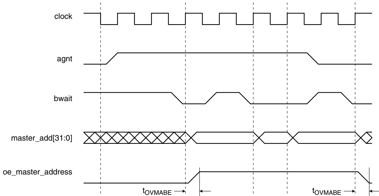
Figure 3. oe_master_address Signal for Atmel AMBA Bus
