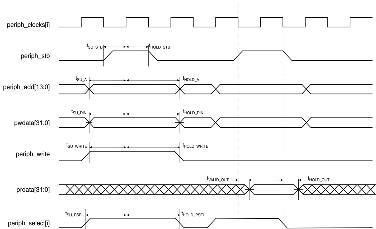
Figure 9. AMBA Peripheral Bus (APB) Interface
