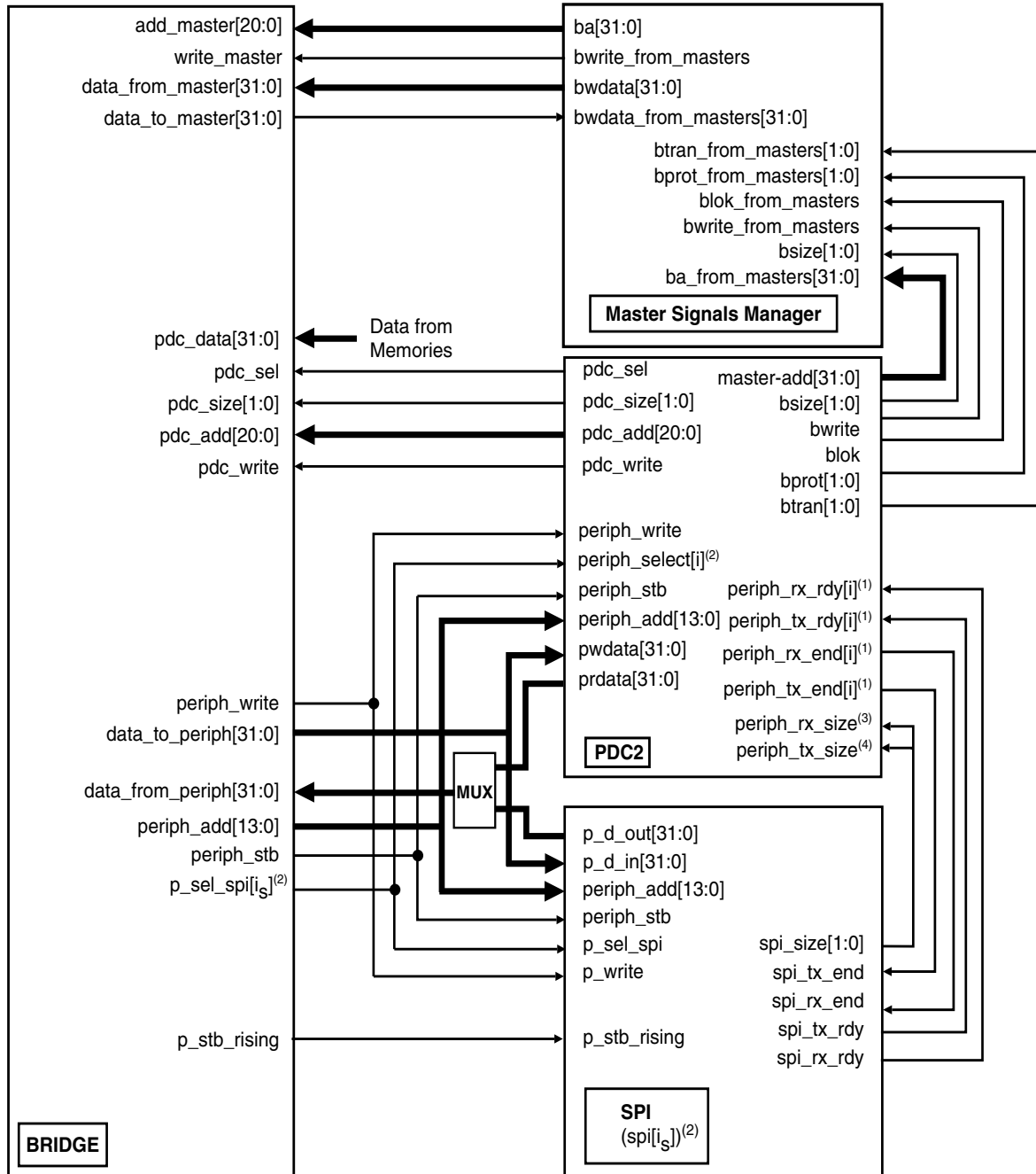
Figure 2. Example of PDC2 Connection with Bridge and SPI
