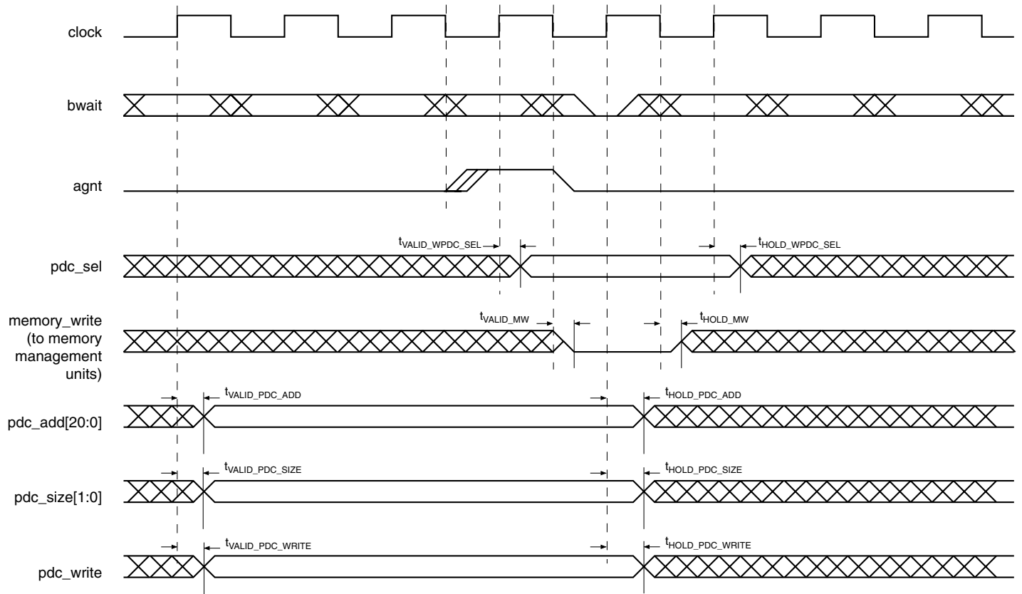
Figure 12. Write APB
