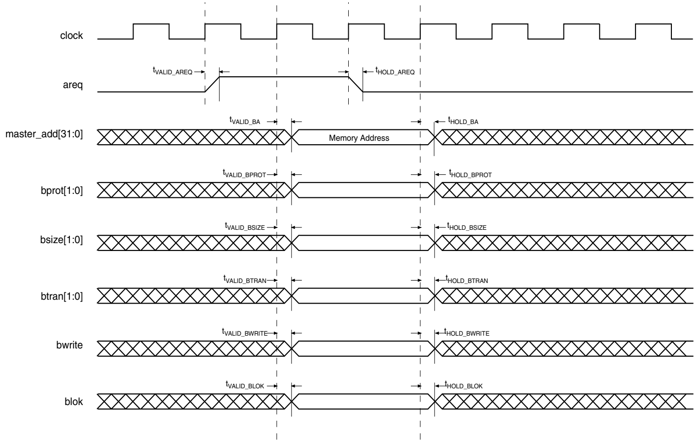
Figure 10. Advanced System Bus (ASB) Dedicated Signals
