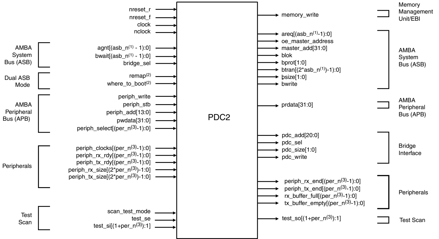
Figure 1. PDC2 Symbol
