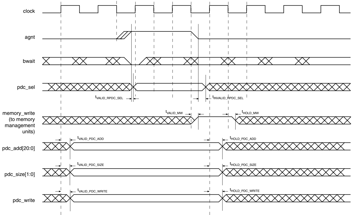
Figure 11. Read APB
