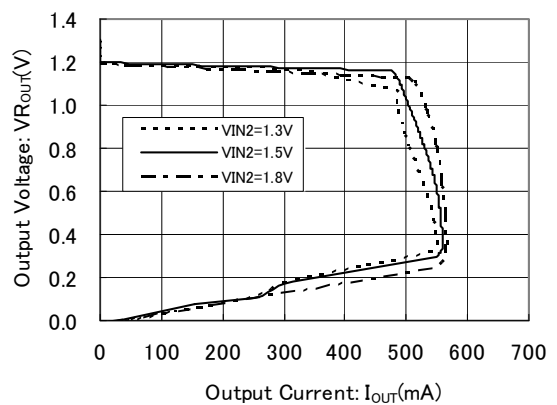
VR OUT =1.2V C IN2 =C BIAS =1.0 μF(ceramic), C L2 =4.7 μF(ceramic) V BIAS =3.6V, Ta=25°C
