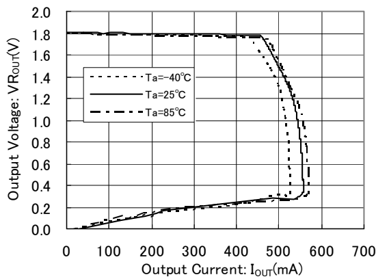
VR OUT =1.8V C IN2 =C BIAS =1.0 μF(ceramic), C L2 =4.7 μF(ceramic) V BIAS =3.6V, V IN2 =2.1V
