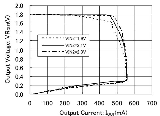
VR OUT =1.8V C IN2 =C BIAS =1.0 μF(ceramic), C L2 =4.7 μF(ceramic) V BIAS =3.6V, Ta=25°C
