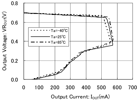
VR OUT =0.7V C IN2 =C BIAS =1.0 μF(ceramic), C L2 =4.7 μF(ceramic) V BIAS =3.6V, V IN2 =1.0V
