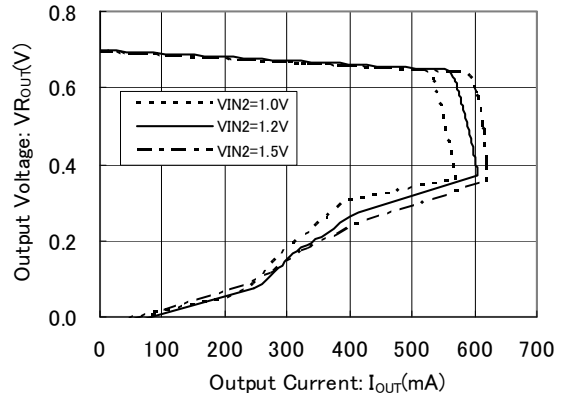
VR OUT =0.7V C IN2 =C BIAS =1.0 μF(ceramic), C L2 =4.7 μF(ceramic) V BIAS =3.6V, Ta=25°C
