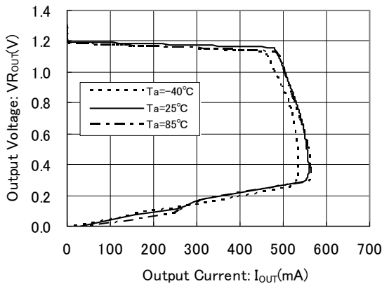
VR OUT =1.2V C IN2 =C BIAS =1.0 μF(ceramic), C L2 =4.7 μF(ceramic) V BIAS =3.6V, V IN2 =1.5V
