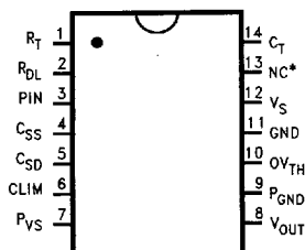
14-Lead Package
