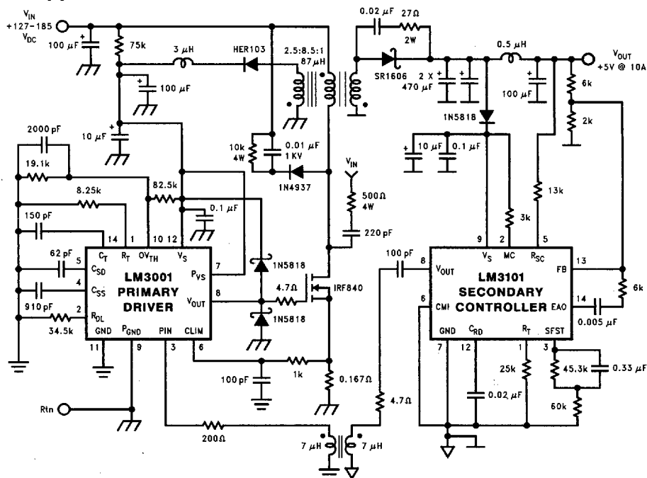
FIGURE 9. Offline Voltage Mode Flyback Regulator
