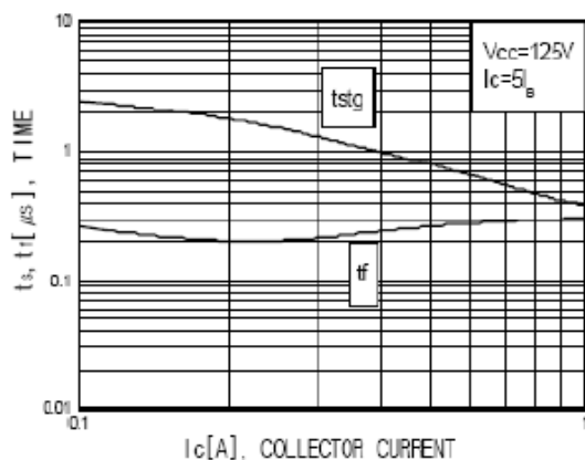
Fig.3 Switching time
