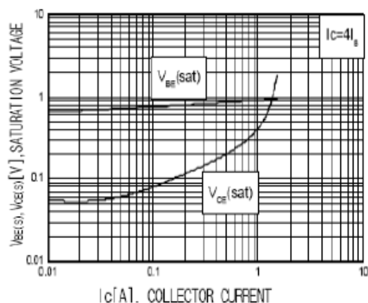
Fig.2 Saturation Voltage
