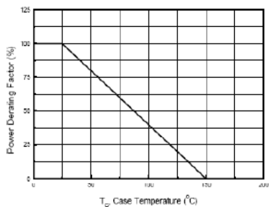
Fig.5 Power Derating
