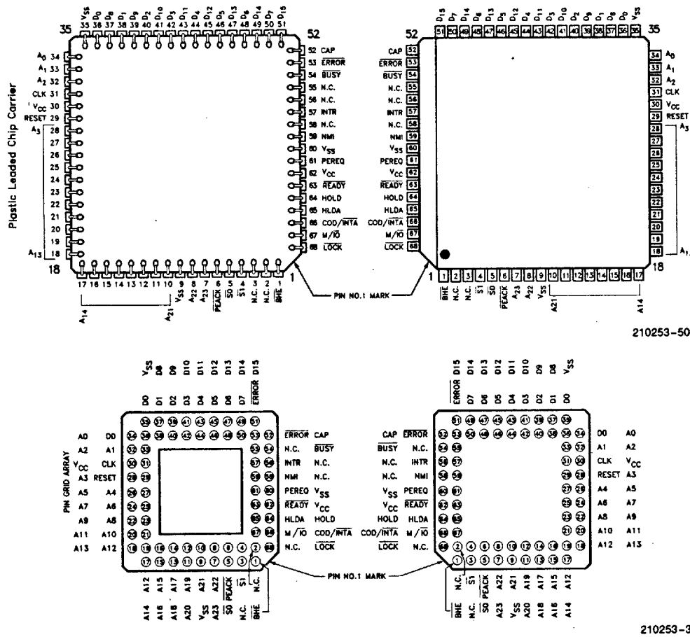
Figure 2. 80286 Pin Configuration
