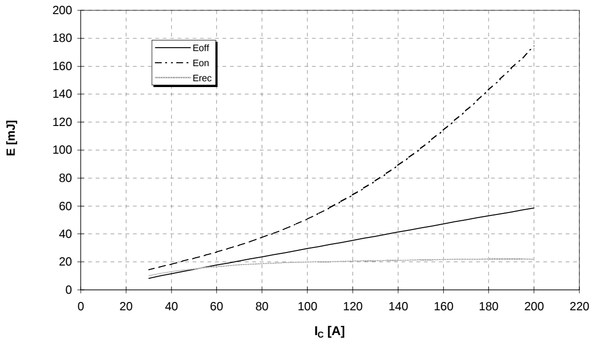
Schaltverluste (typisch) E_{on} = f(I_C) , E_{off} = f(I_C) , E_{rec} = f(I_C) Switching losses (typical) R_{gon} = R_{goff} \approx 15\Omega , V_{CE} = 900V , T_j = 125^\circ C
