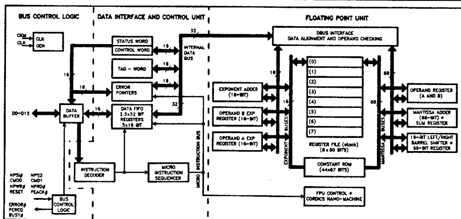
Figure 0.1. Intel287™ XL MCP Block Diagram
