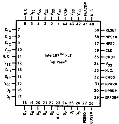
Figure 3.2. PLCC Pin Configuration
