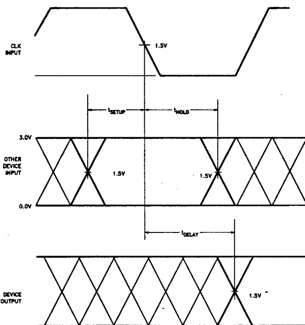
Figure 4.2. AC Setup, Hold, and Delay Time Measurements—General
