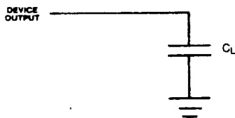
Figure 4.3. AC Test Loading on Outputs
