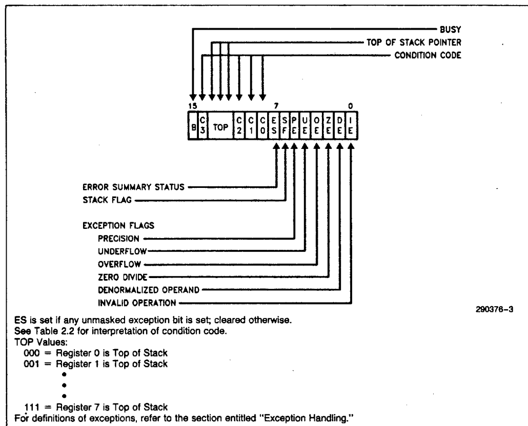
Figure 2.2. Status Word
