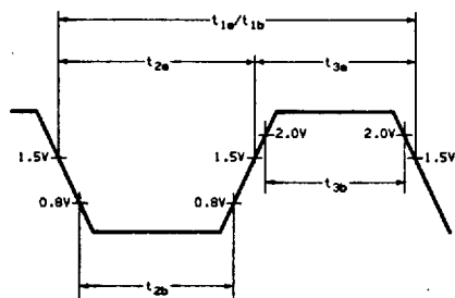
Figure 4.1. AC Drive and Measurement Points—CLK Input
