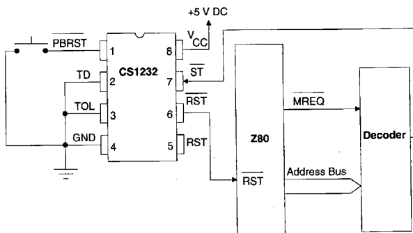
Figure 2. Watchdog Timer
