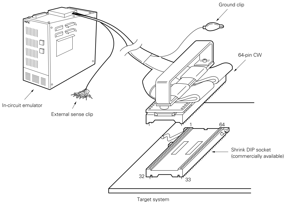
Figure 2-3. Connecting EP-78024CW-R and Target System
