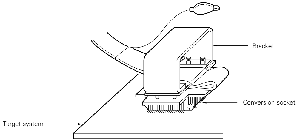
Figure 2-7. Removing EP-78024GF-R
