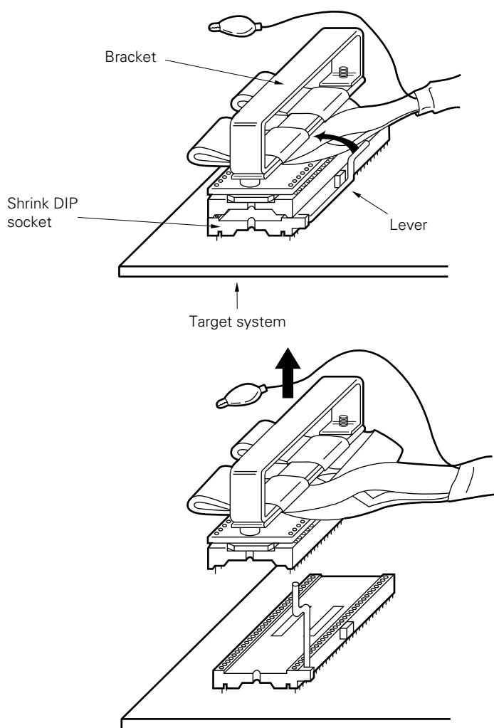
Figure 2-6. Removing EP-78024CW-R
