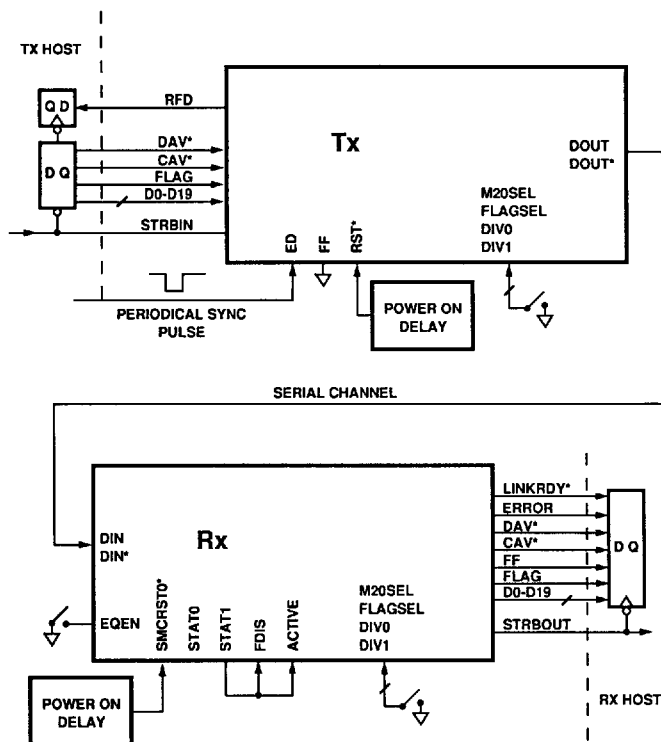
Figure 17. Simplex Configuration.
