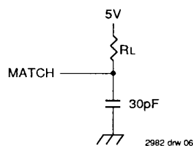
Figure 3. Output Load for MATCH
