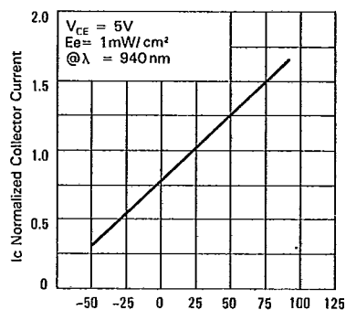
FIG. 2 NORMALIZED COLLECTOR CURRENT VS AMBIENT TEMPERATURE
