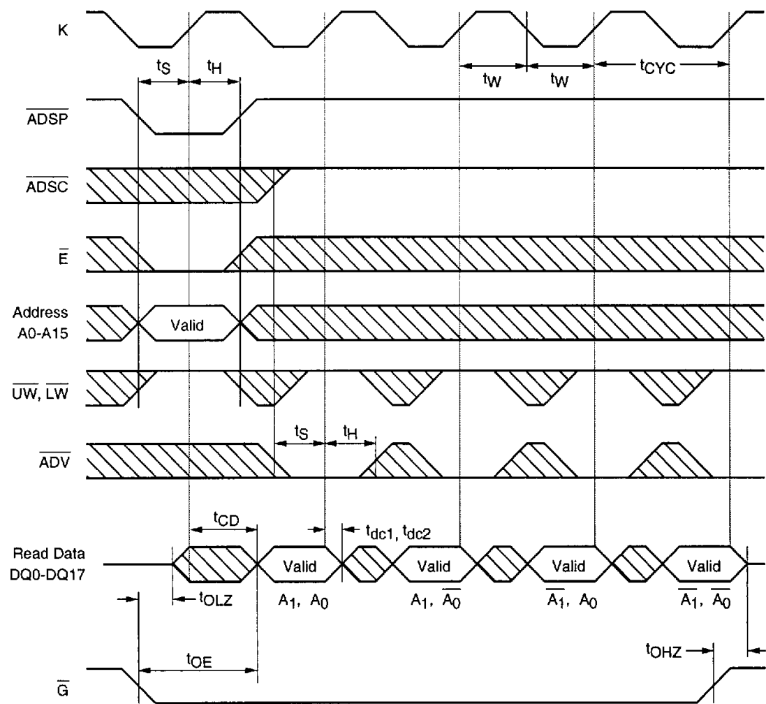
ADSP Read Timing Diagram
