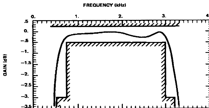
Rx HIGH-PASS FILTER TYPICAL RESPONSE AND LIMITS CHART (HP : f_s = 72\text{kHz} , LP : f_s = 288\text{kHz} )
