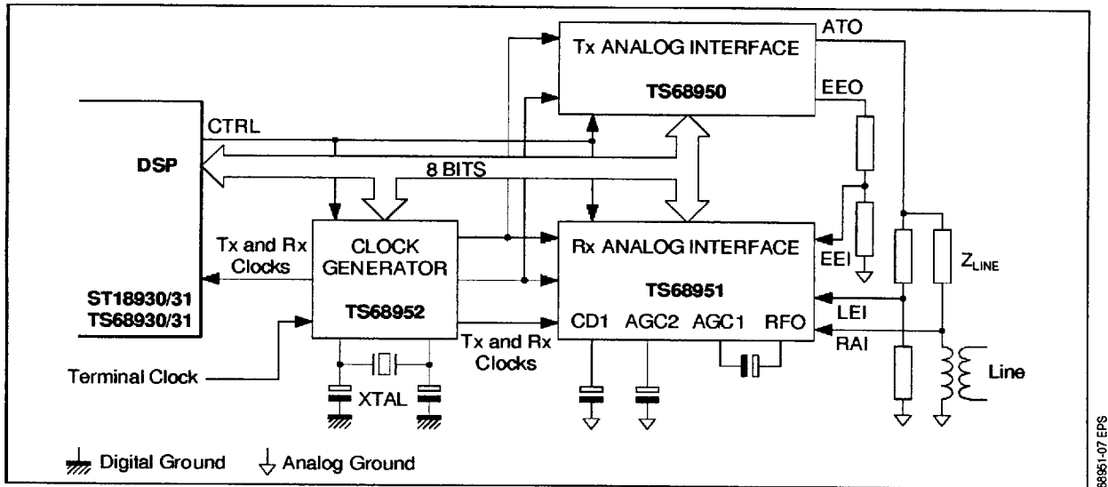
Figure 4 : Modem Analog Front-end Chip Set
