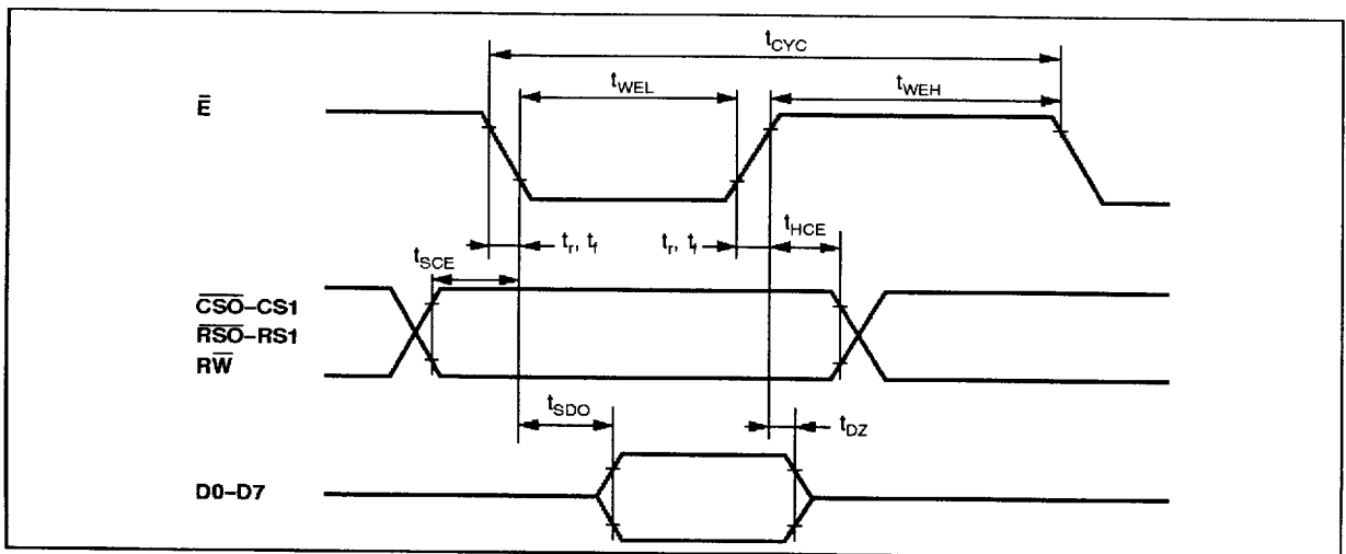
Figure 3 : Read Operation
