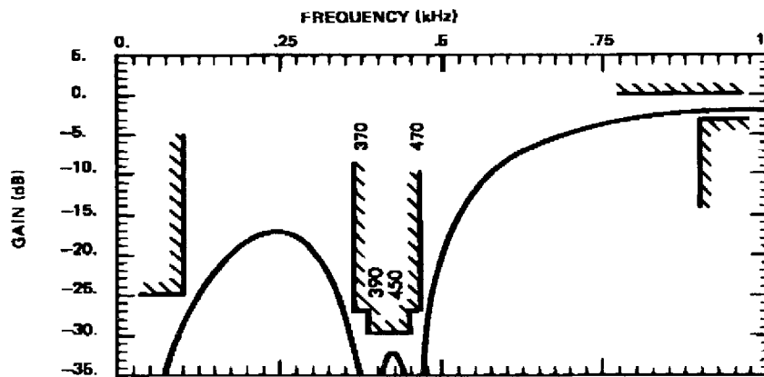
Rx BAND-PASS FILTER TYPICAL RESPONSE FOR V.22 MODE (Low Channel) (HP : f_s = 72\text{kHz} , LP : f_s = 144\text{kHz} )
