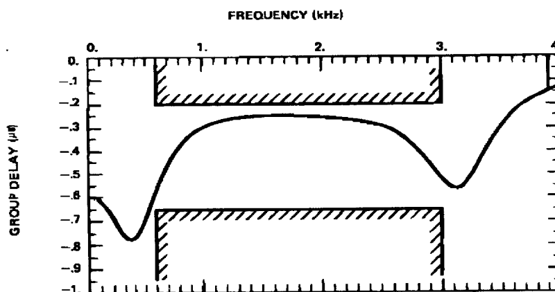
Rx LOW-PASS FILTER TYPICAL GROUP DELAY TIME AND LIMITS CHART ( f_s = 288\text{kHz} )
