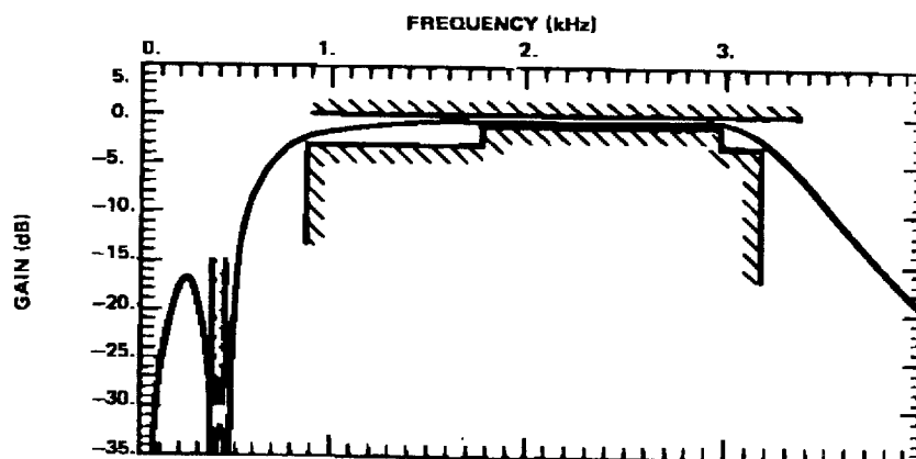
Rx BAND-PASS AND REJECTION FILTER TYPICAL RESPONSE AND LIMITS CHART (HP and REJ. : f_s = 72\text{kHz} , LP : f_s = 288\text{kHz} )
