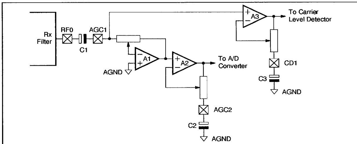
Figure 1 : Rx Amplifiers Schematic
