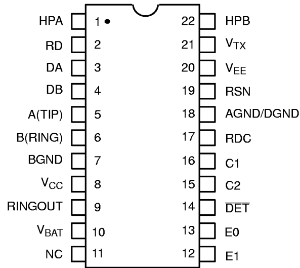
22-Pin Ceramic DIP
