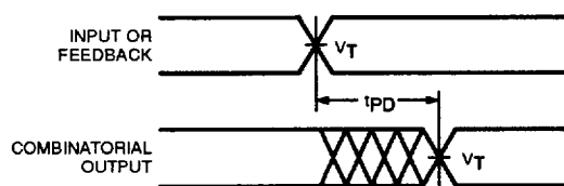
Combinatorial Output
