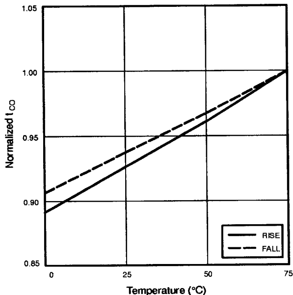
Normalized t_{CO} vs Temperature ( V_{CC} = 3.3V , output capacitance = 50pF, 5 outputs switching)
