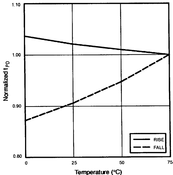
Normalized t_{PD} vs Temperature ( V_{CC} = 3.3V , output capacitance = 50pF, 5 outputs switching)
