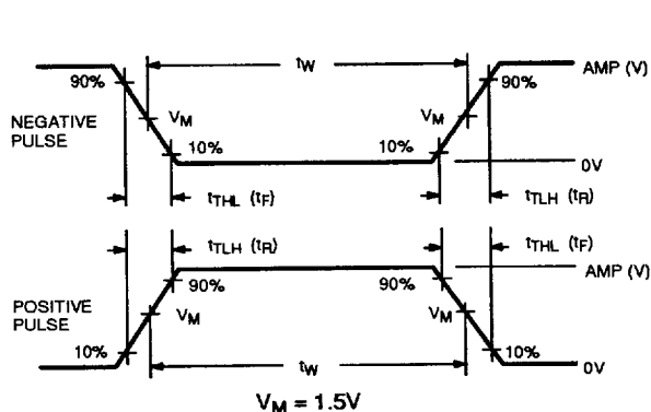
Input Pulse Definition
