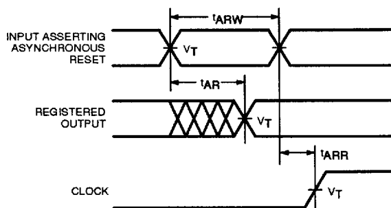
Asynchronous Reset
