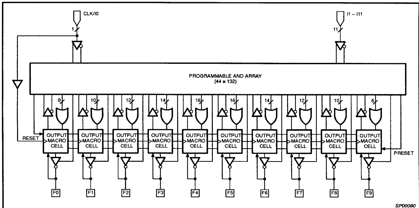
Figure 1. Functional Diagram
