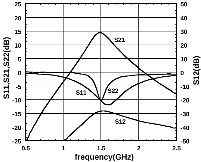
S11,S21,S22 Vs. frequency
